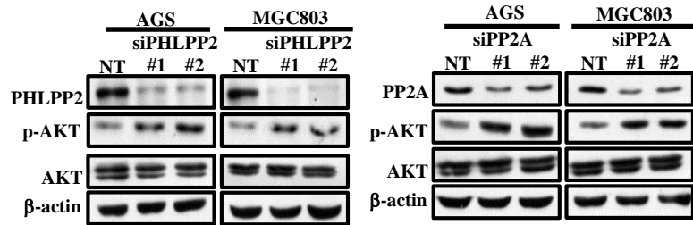
Supplementary Fig. S1. Western blot analysis of expression of p-AKT and total AKT in the AGS and MGC803 cells with either PHLPP2 or PP2A knockdown using two specific siRNAs.
