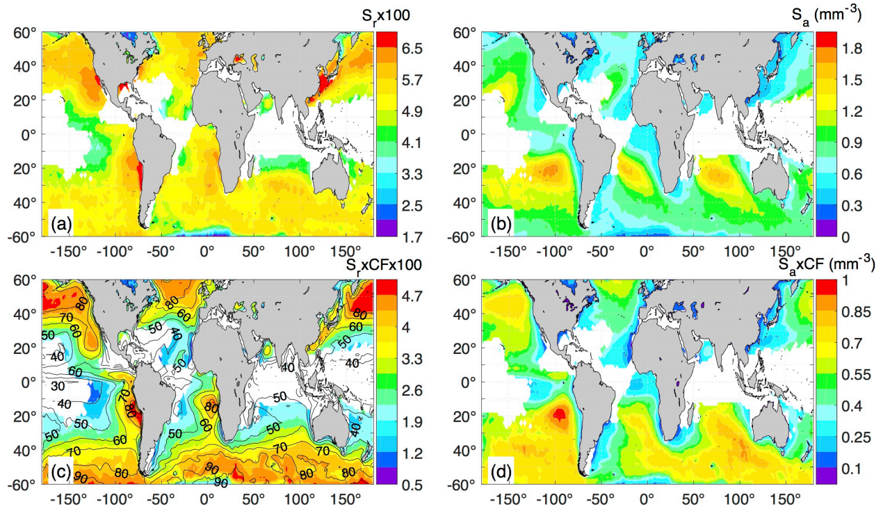
Figure S5: Annual values of a) albedo relative susceptibility, b) absolute albedo susceptibility, c) as in a) but multiplied by cloud fraction, d) as in b) but multiplied by cloud fraction.
