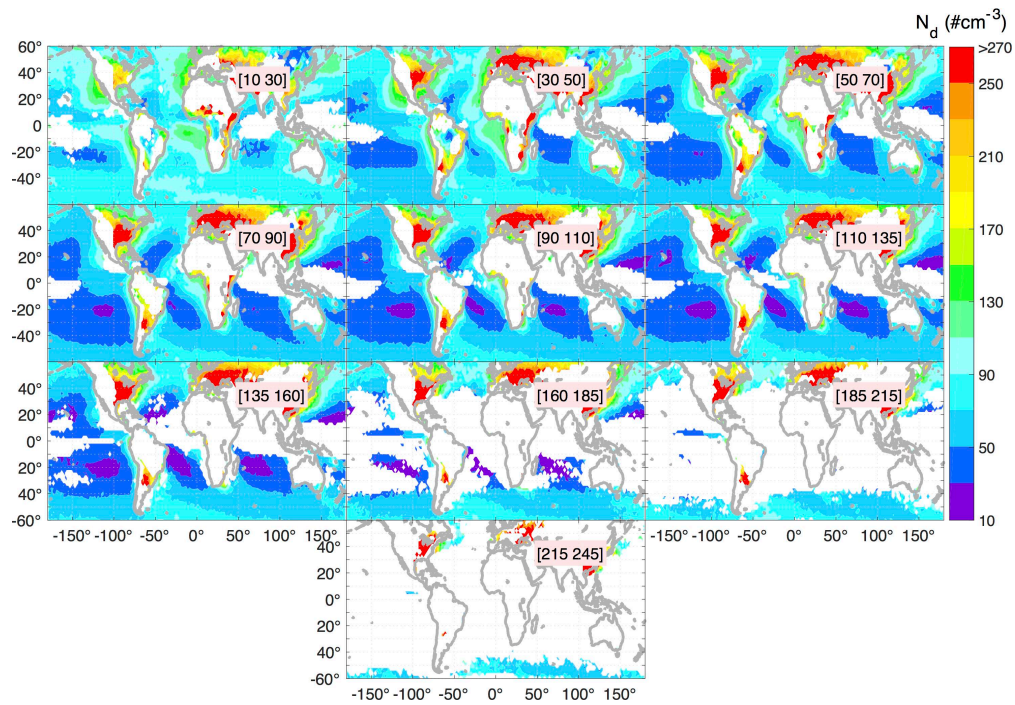
Figure S4: Seasonally averaged N_d for the 10 LWP bins utilized in this study.
