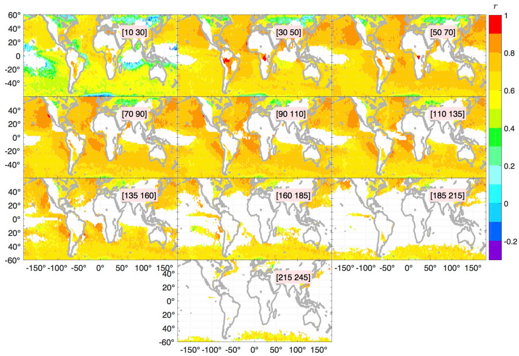
Figure S1: Seasonally averaged linear correlation coefficient between albedo A and \ln(N_a) for the 10 LWP bins utilized in this study.
