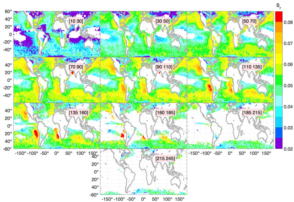
Figure S2: Seasonally averaged relative susceptibility for the 10 LWP bins utilized in this study.
