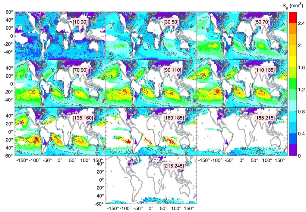
Figure S3: Seasonally averaged absolute susceptibility for the 10 LWP bins utilized in this study.
