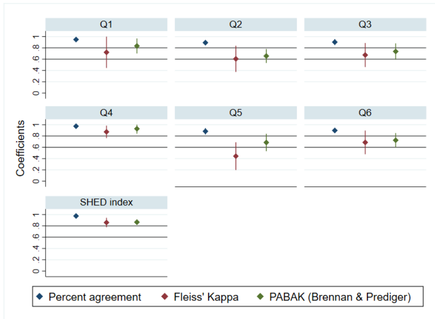
Figure 1: Inter-rater reliability calculations for individual items and SHED index
