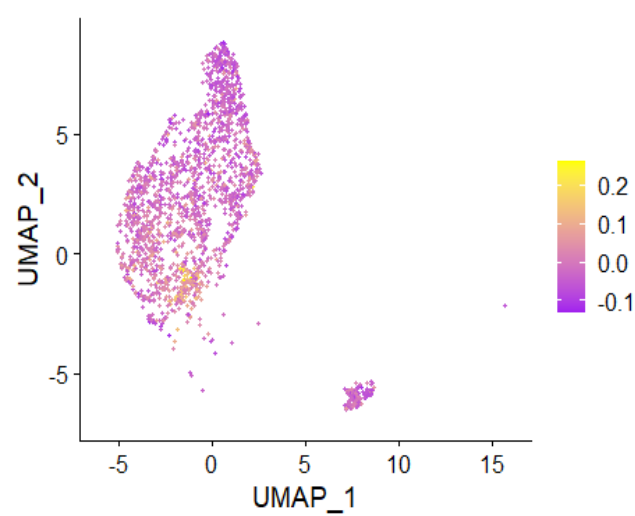
Non-Inflammatory Module (69 genes)
