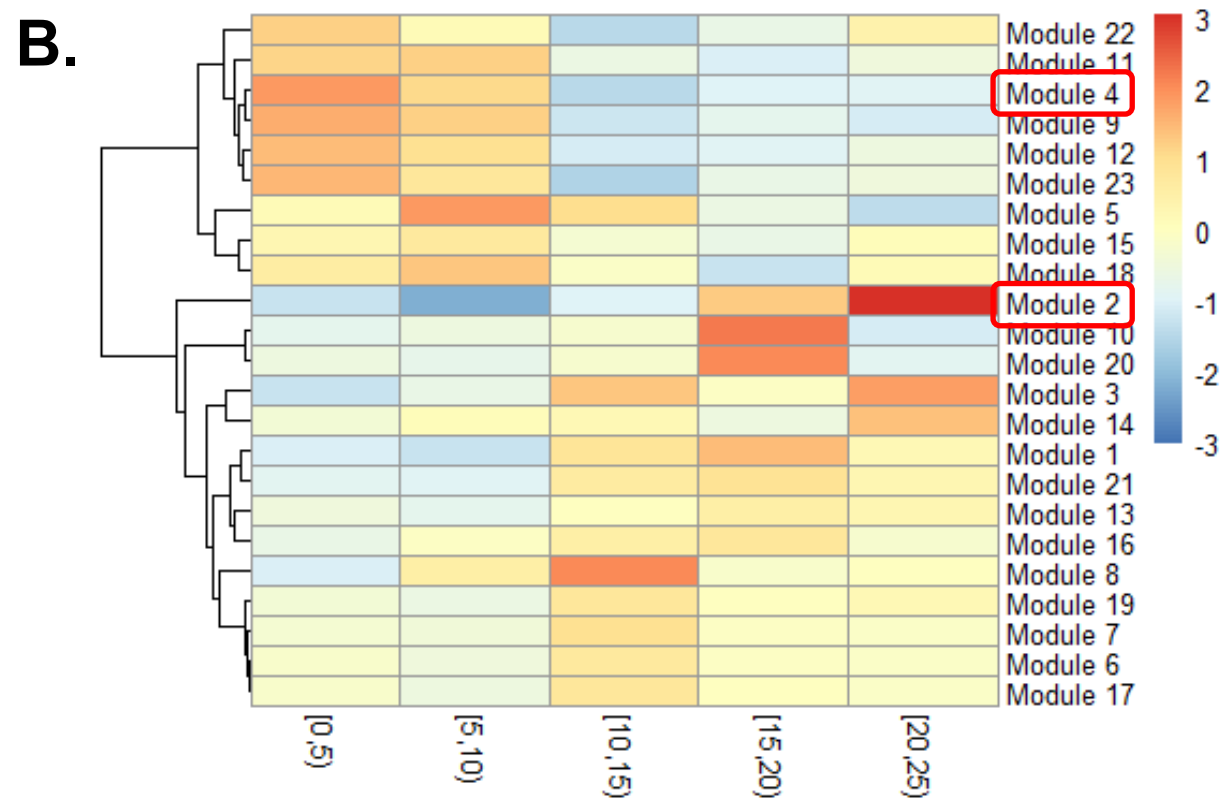
Non-Inflammatory Module (69 genes)
