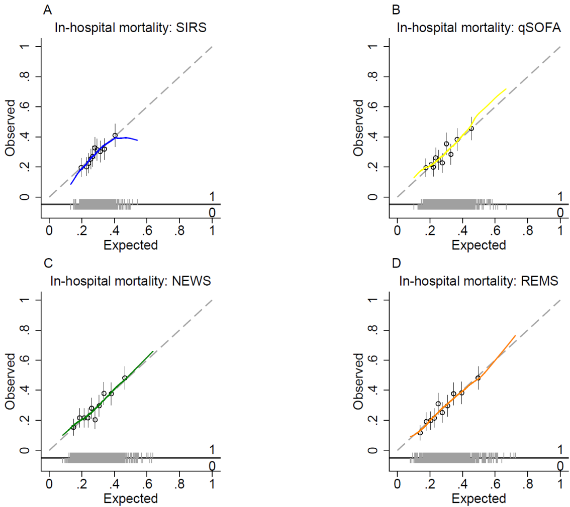
Figure S4. Calibration plots of baseline risk model plus early warning scores for in-hospital mortality in patients with suspected sepsis.
