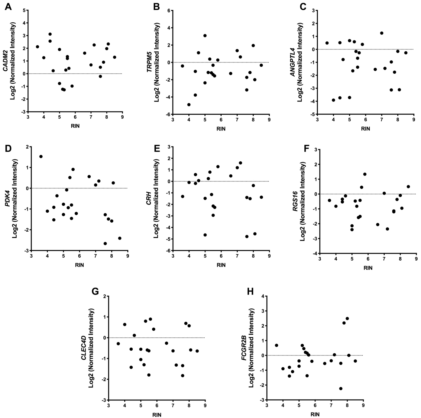
Supplementary Fig. 3. Expression of genes that are differentially expressed in the pancreata of AA+ individuals vs. control, as measured by microarray analysis and shown relative to the RIN value of each sample.
