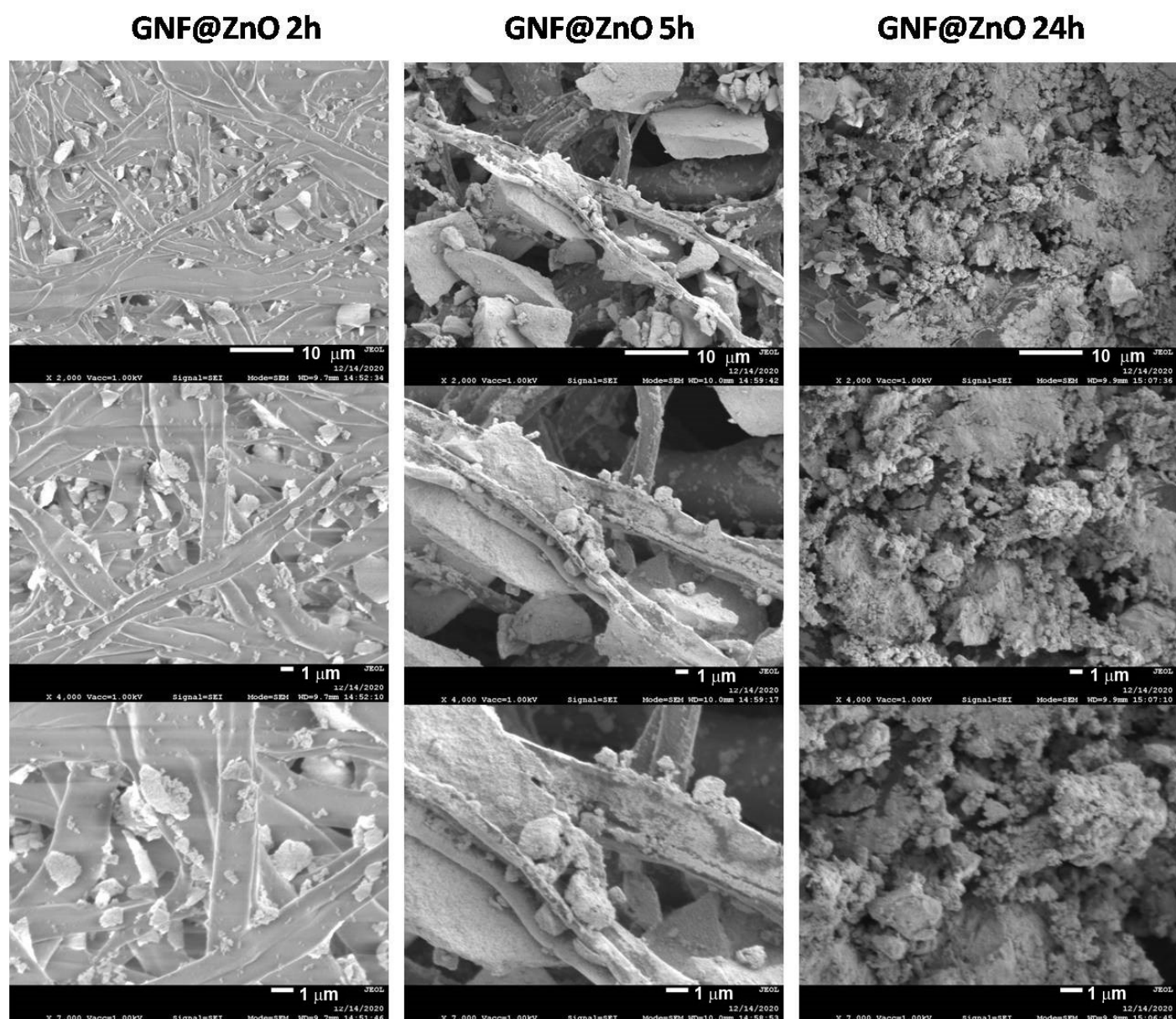
Figure S1. SEM images (magnification \times 2000 , \times 4000 and \times 7000 ) of GNF@ZnO 2h, GNF@ZnO 5h and GNF@ZnO 24h.
