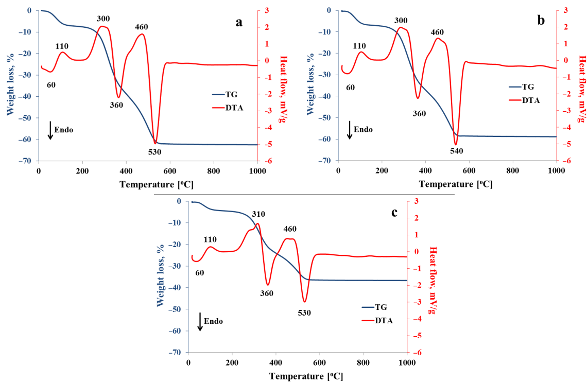
Figure S2. TG-DTA curves of GNF@ZnO 2h (a), GNF@ZnO 5h (b) and GNF@ZnO 24h (c).
