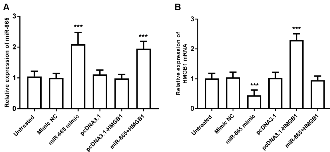
Figure S1. Transfection efficiency was confirmed using reverse transcription-quantitative PCR. (A) miR-665 mimic significantly promoted the expression of miR-665. (B) miR-665 mimic significantly inhibited the expression of HMGB1 mRNA, pcDNA3.1- HMGB1 promoted the expression of HMGB1 mRNA. *** P < 0.001 vs. untreated cells. miR, microRNA; NC, negative control; HMGB1, high mobility group box 1.
