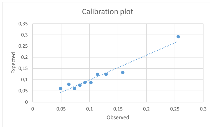
Supplemental Figure 1. Calibration plot of the clinical prediction rule for repeated consultations with functional somatic symptoms
