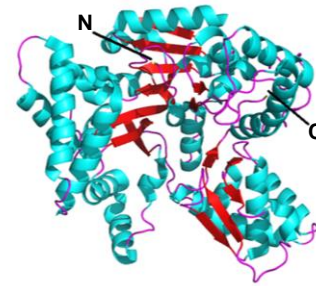
C PKMT1 ( Rickettsia prowazekii )
