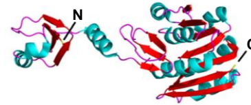
F PrmA ( Thermus thermophilus )
