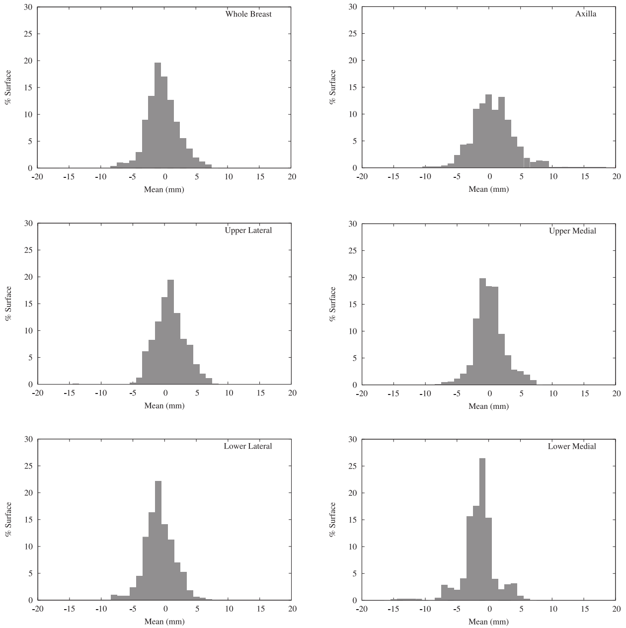
Supplementary 1. Histograms of the mean difference between the planning CT scan and follow-up CBCT scans over the course of treatment (i.e., inter-fractional shape changes) for the different ROIs. Each bar indicates the proportion of the surface area in the ROI that exhibits the corresponding uncertainty.
