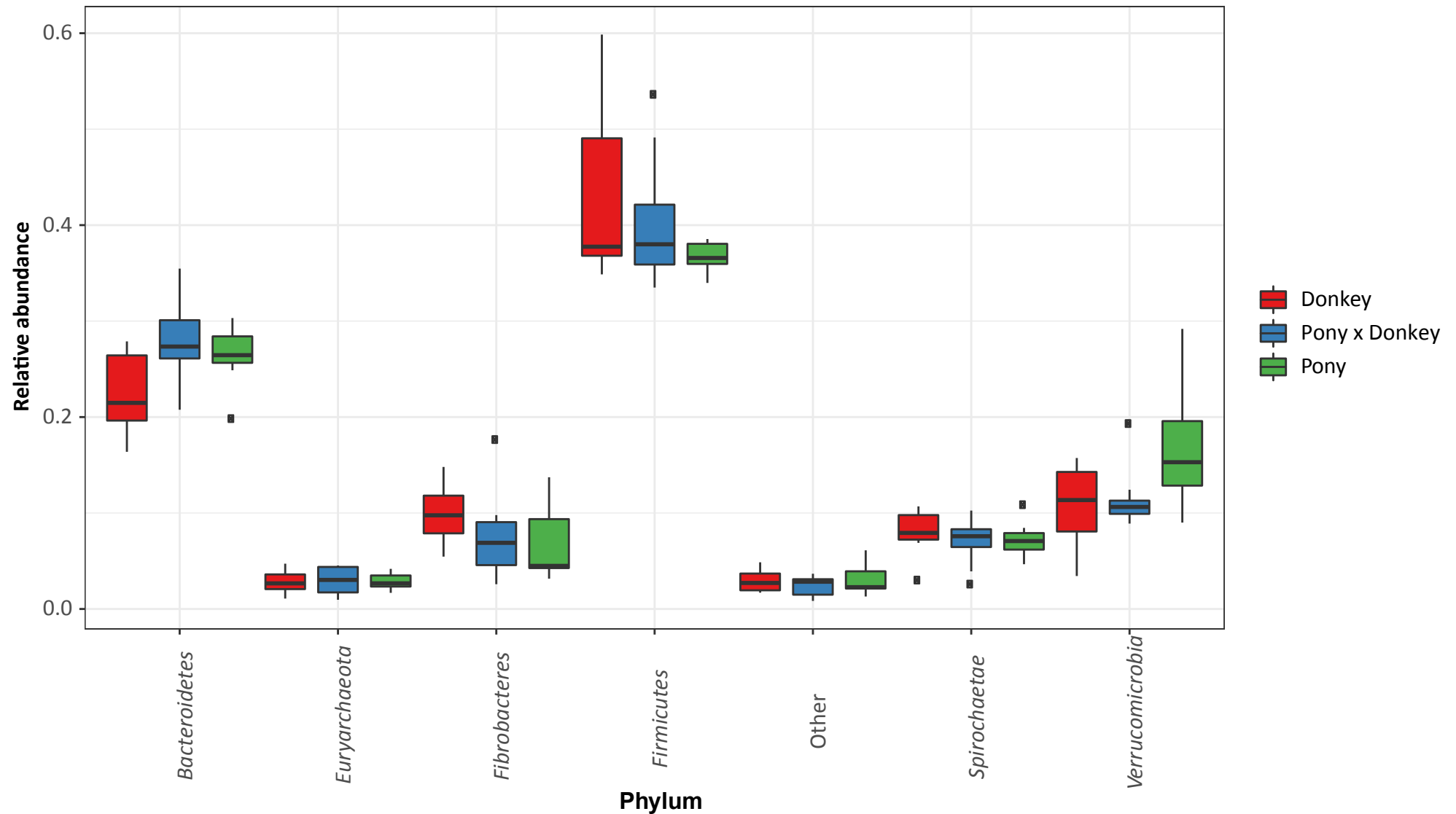
Figure S1. Boxplot showing the six main bacterial and archaeal phyla detected in the different equine types. The minor phyla (<1%) are grouped as 'Other'. Boxes show the 25th and 75th percentiles with the median represented by a horizontal line. Whiskers show the data range with the exception of any outliers, which are indicated as data points.
