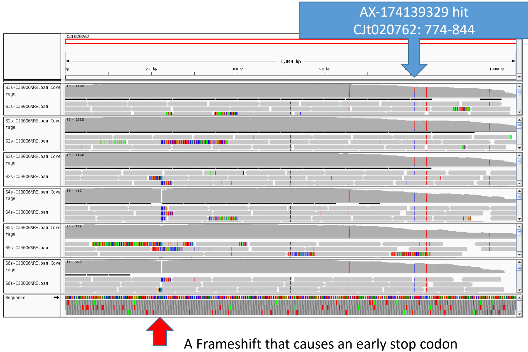
Figure S2 A 4bps deletion and a SNP marker in CJt020762.
