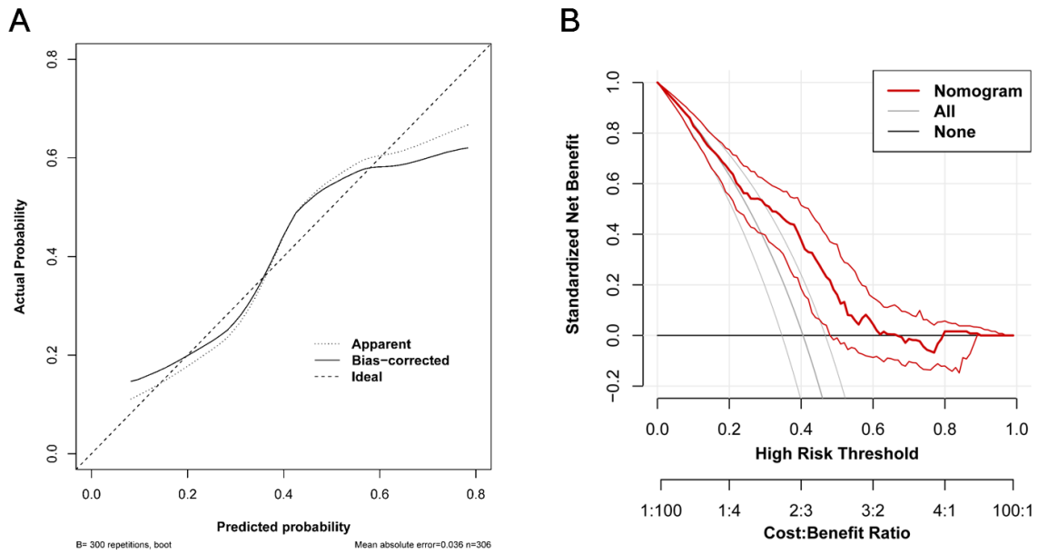
S3 Fig. (A) Calibration curve of the nomogram predicting the probability of pathologic complete response (pCR). The x-axis and y-axis show the predicted and actual probabilities of pCR, respectively. (B) Decision curves of the nomogram predicting pCR. The x-axis and y-axis indicate the threshold probabilities and the net benefit, respectively.
