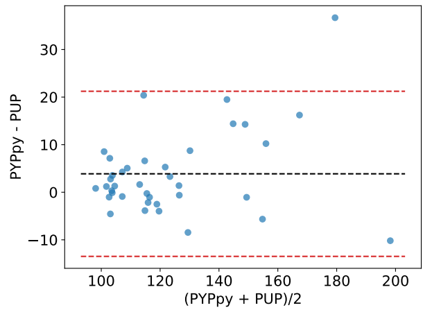
(f) Arousal threshold
