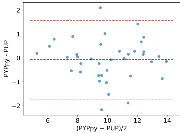
(e) Circulatory delay ( \delta )
