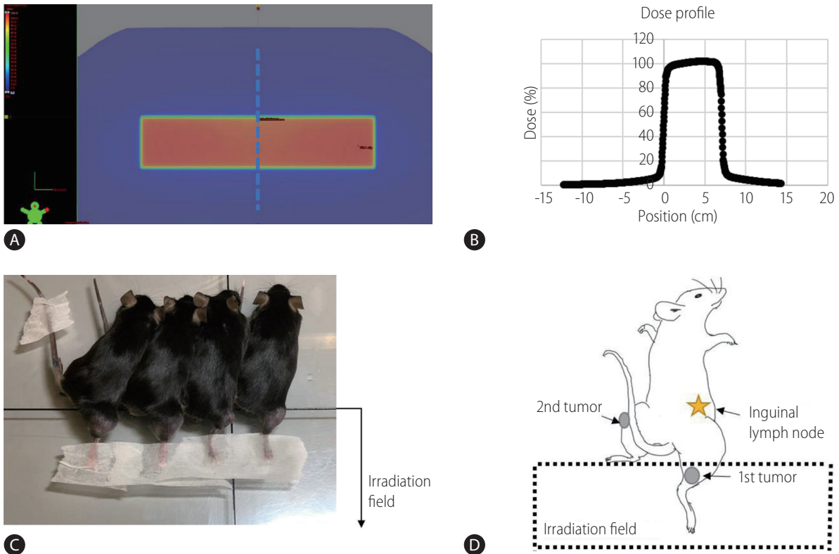
Supplementary Figure 1. Setup for irradiation of Hepa 1–6 tumors implanted in C57BL/6 mice. (A) A treatment plan for making 30x7 cm field size. (B) Cross-sectional dose distribution. (C) Photo image showing that tumor-bearing right hind legs were located within the irradiation field. (D) Schematic diagram illustrating position of two tumors and a tumor-draining inguinal lymph node. A primary tumor implanted into a right leg was exposed to X-ray irradiation, but the left leg harboring secondary tumor and the inguinal lymph node were not included in the radiation field.
