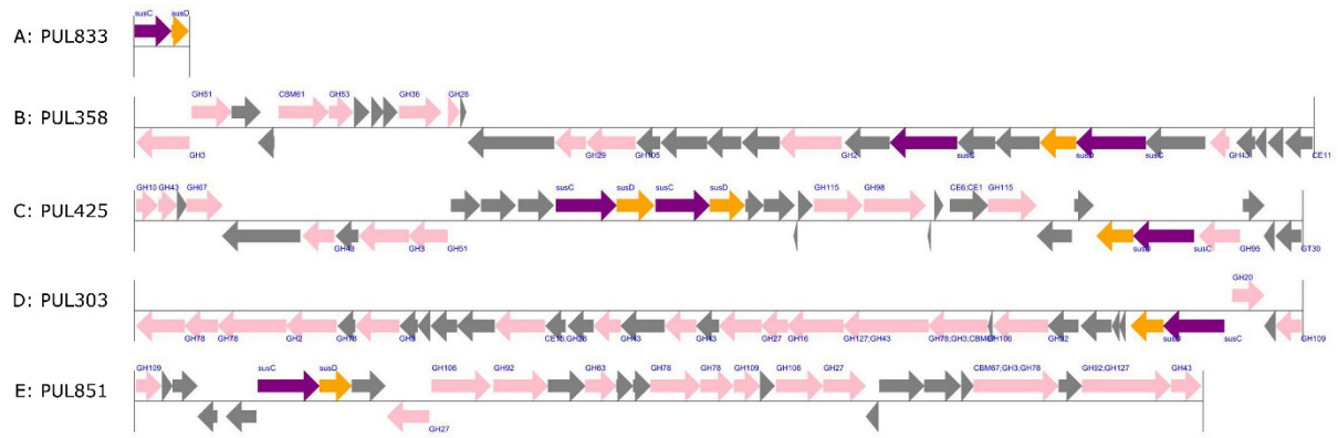
Supplementary fig 1: Several predicted polysaccharide utilisation loci (PULs). A: The most common PUL consisting of only a susC/D pair. B-E: The 4 largest PULs identified in our dataset.
