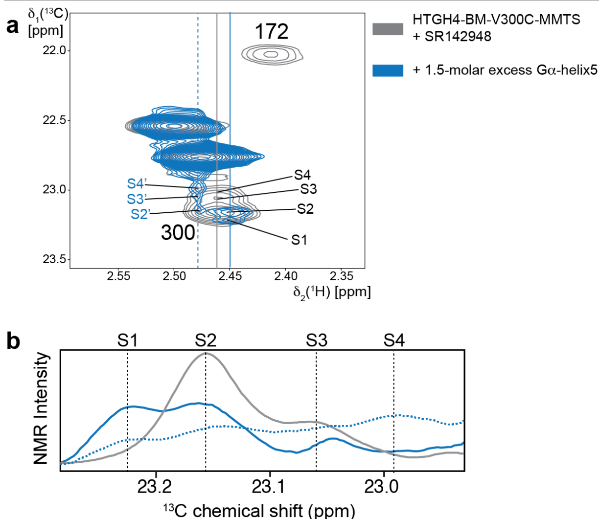
Figure S3. NMR titration of ^{13}\text{C} -MMTS-labeled HTGH4-BM-V300C in the antagonist bound form (SR142948) with a peptide derived from the C-terminal helix 5 of a G\alpha_{i,1} subunit. (a) 2D- [^{13}\text{C}, ^1\text{H}] -HMQC experiments of both states reveals marked differences in signal intensity and chemical shifts for amino acid residues close to the cytoplasmic G-protein coupling interface (residues 172 and 300). HTGH4 binds to the G-protein even in the antagonist-bound form leading to complete line broadening at position 172 and chemical shift perturbations as well as changes in signal intensity at position 300. (b) Slices along the axes in the ^{13}\text{C} dimension indicated in panel (a) show that mostly the S2 state and to some extent the S3 state is populated in complex with the antagonist (grey line). Upon addition of the G-protein peptide we observe a splitting of the NMR resonances according to the indicated states. One set of signals corresponding to the S1 and S2 states remain at a similar position as observed without the peptide (blue line). In addition, a second set of signals appears at a different ^1\text{H} frequency (broken blue line). There, the active states S3 and S4 are populated to a higher extent, suggesting that these signals originate from the G-protein-bound species. In order to distinguish between the two sets of signals, we denote these as S1-S4 and S1'-S4'. These data indicate that there is an equilibrium between free and G-protein bound receptor in slow exchange giving rise to two sets of NMR signals. The free form adopts mostly the inactive states, whereas the G-protein-bound form is predominantly present in the active conformation.
