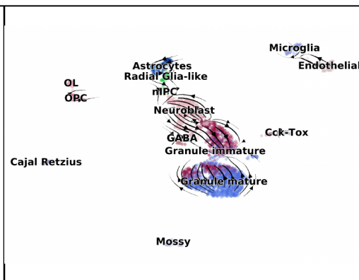
alevin_spliced_unspliced_gtr
