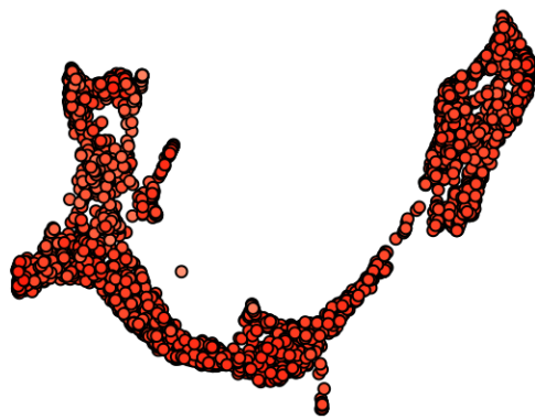
alevin_spliced_unspliced_gtr
