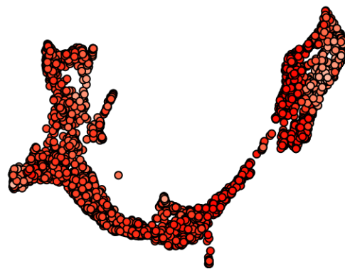
droptest
