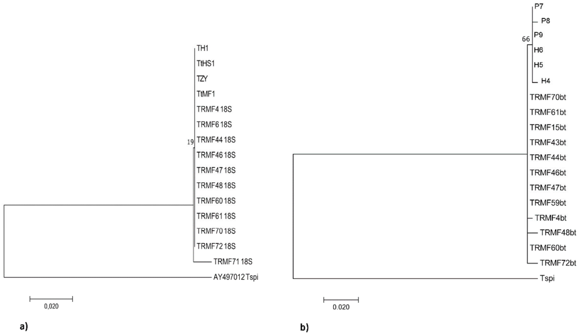
Figure S1. ML trees elaborated from the Dataset_18S ( a ) and the Dataset_btub ( b ) showing the evolutionary relationships of Trichuris spp. included (see Table 2). Bootstrap values are reported at nodes.
