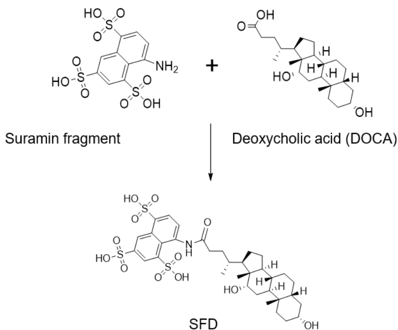
Figure S1. Synthetic scheme of suramin fragment and deoxycholic acid conjugate (SFD). Suramin fragment was conjugated to deoxycholic acid (DOCA) in one step.
