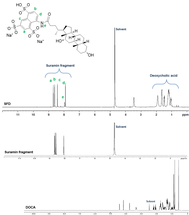
Figure S2. 1 H-NMR spectra of SFD (deuterium oxide as solvent), suramin fragment (deuterium oxide as solvent) and DOCA (dimethyl sulfoxide-d 6 as solvent) (500 MHz).
