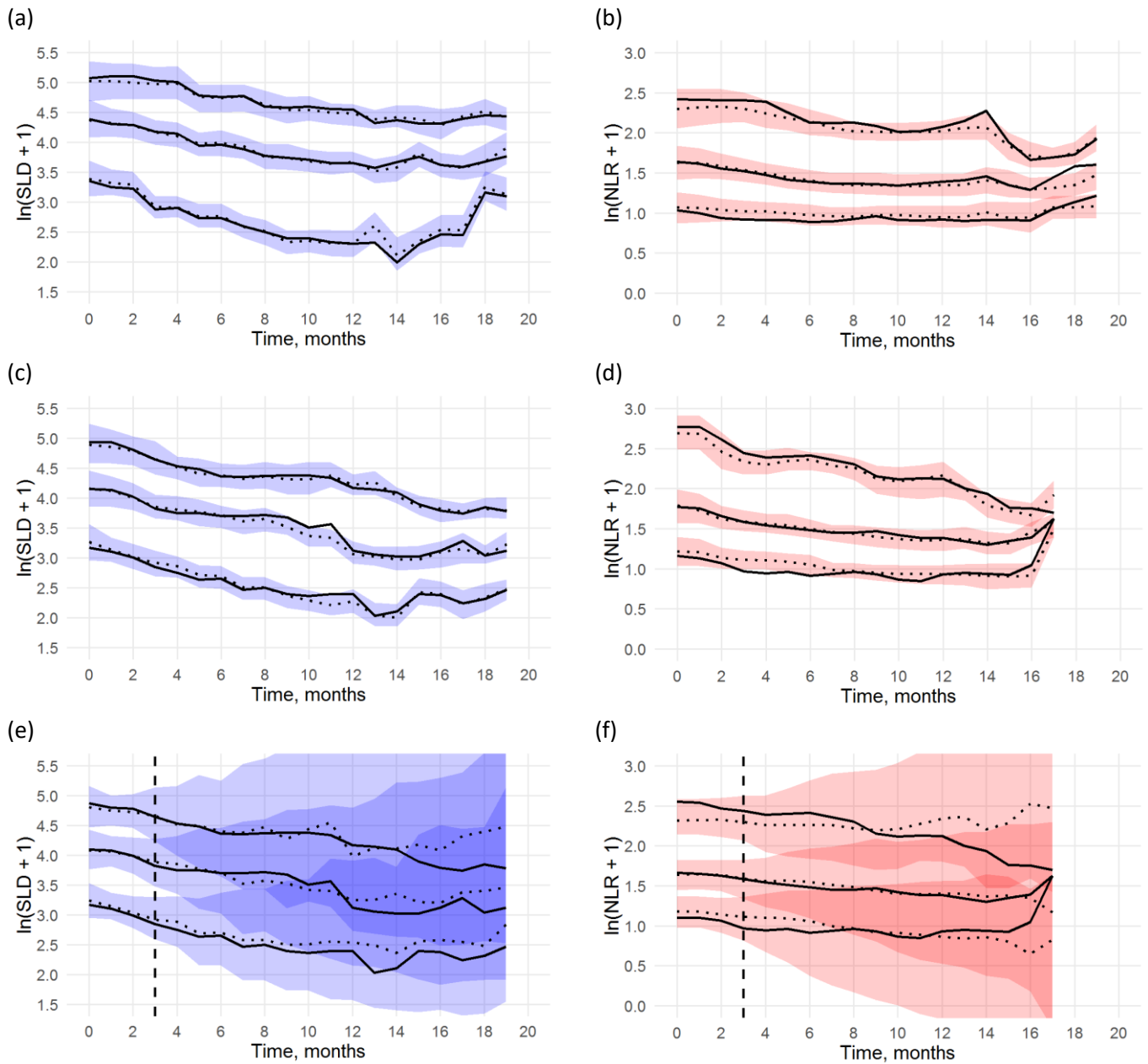
Figure S3. a) and b): VPC diagnostics for the longitudinal data (training dataset). c) and d): VPC diagnostics estimated on the validation dataset. e) and f): Model predictions of longitudinal profiles, based on limited data (3 months of longitudinal data). Solid lines: Median, actual, with 90% and 10% quantiles of longitudinal data. Dotted lines: Predicted values; range in color: 95% CI of predictions.
