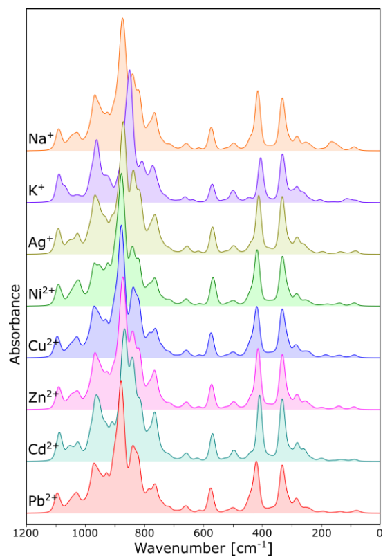
Figure S2. IR spectra of FAU calculated for "B" model
