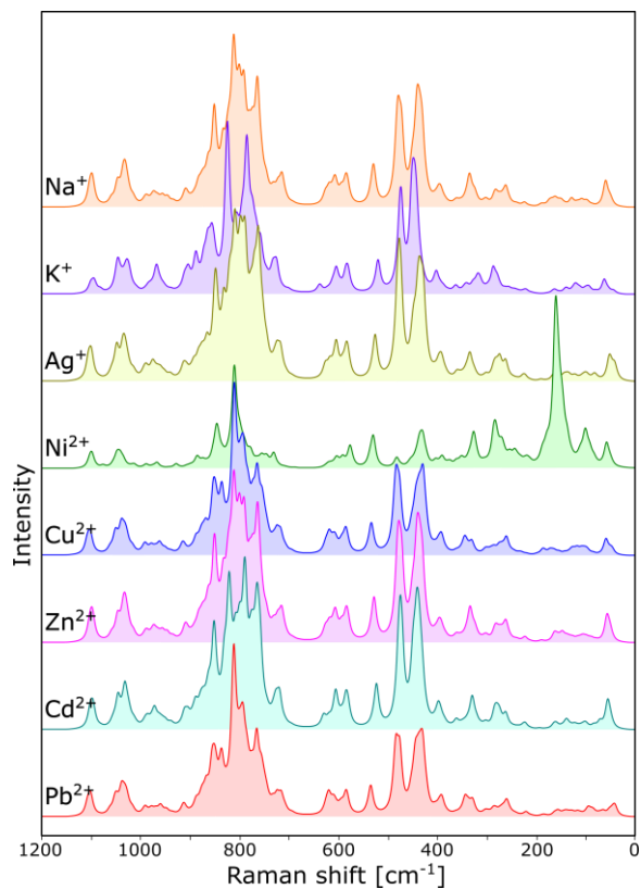
Figure S5. Raman spectra of FAU calculated for "B" model
