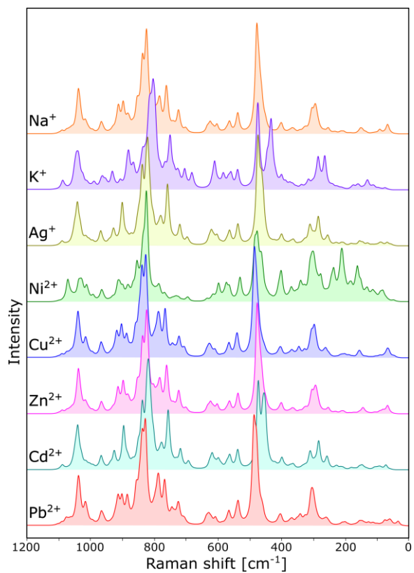
Figure S4. Raman spectra of FAU calculated for "A" model
