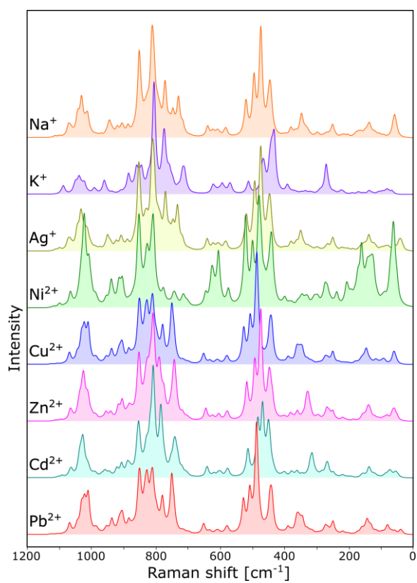
Figure S6. Raman spectra of FAU calculated for "C" model
