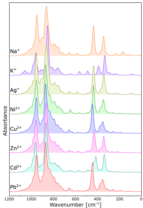
Figure S3. IR spectra of FAU calculated for "C" model
