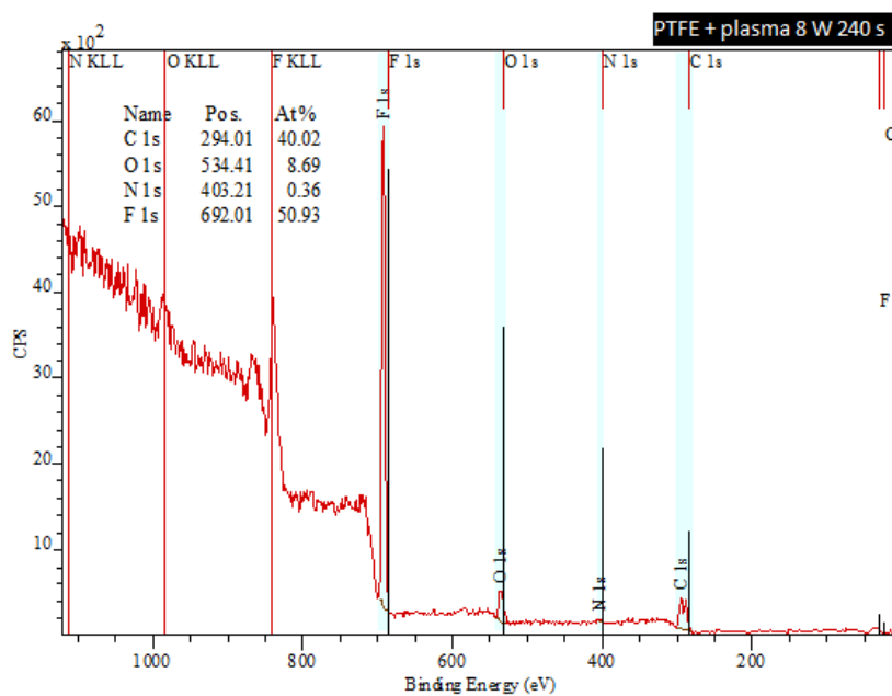
Figure S1. XPS spectra of a pristine PTFE and plasma-treated PTFE sample at 8 W for 240 s.
