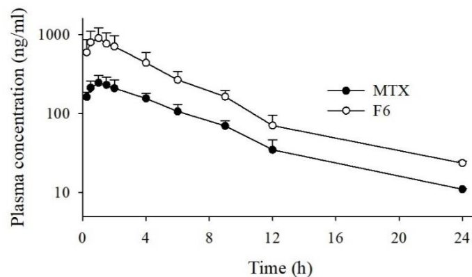
Figure S1. Plasma concentration (log scale)–time profiles of MTX after oral administration of free drug or F6 formulation in rats.
