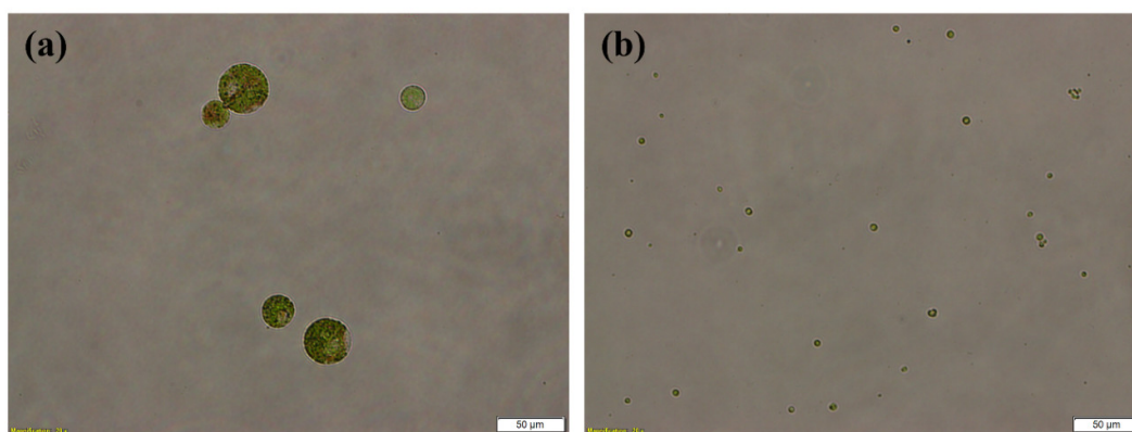
Figure S1. A microscopic image of algal cells obtained from each of (a) outlet 2 and (b) outlet 6 after 7 days of cultivation. Scale bar = 50 \mu\text{m} .
