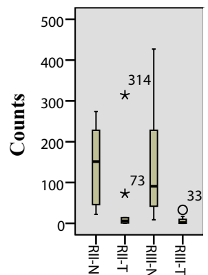
WT1_AS
