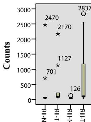
RPL10P9
