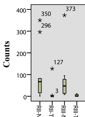
MTDHP3
