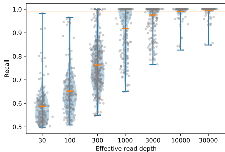
Required relationships for dataset with noise and 20 subclones
