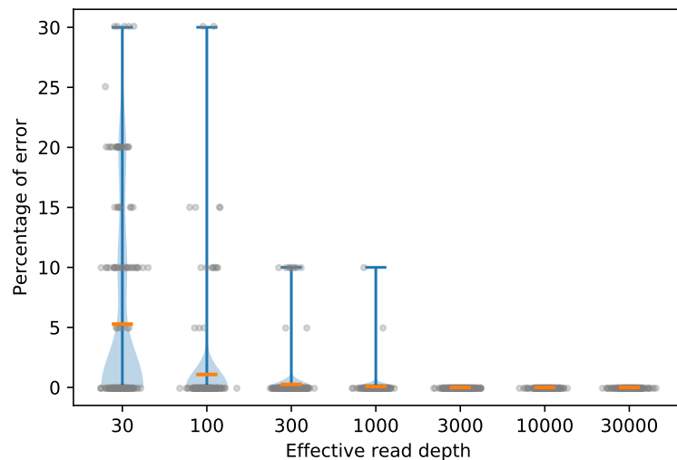
Differently defined error for dataset with noise and 5 subclones
