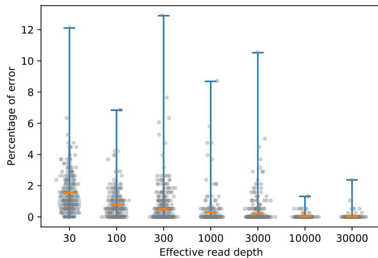
Differently defined error for dataset with noise and 20 subclones
