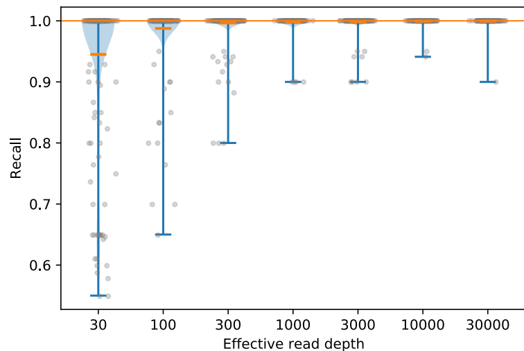
Required relationships for dataset with noise and 5 subclones
