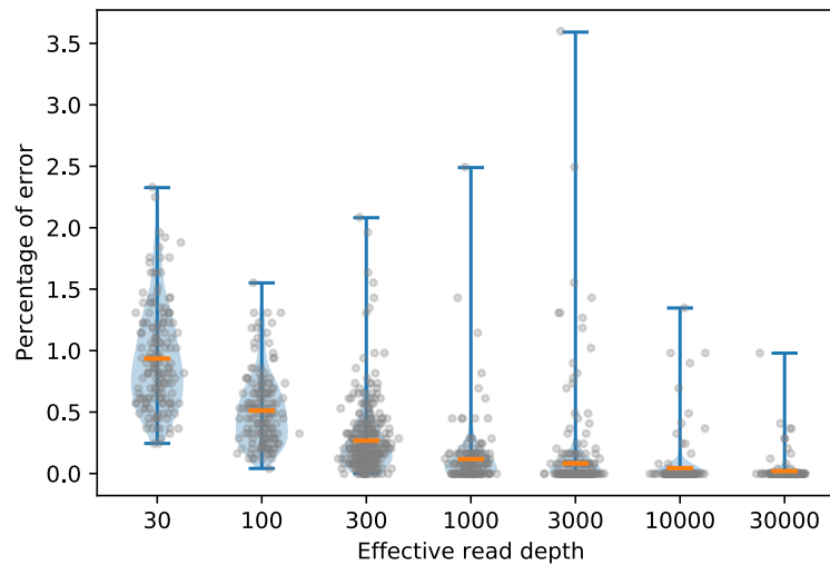
Differently defined error for dataset with noise and 50 subclones
