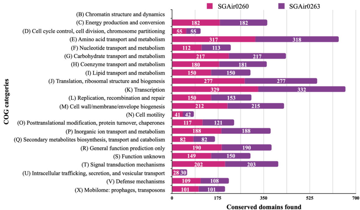
Additional File 6. Horizontal bar chart showing COG categories and number of conserved domains found for each category in the genomes of Bacillus cereus strains SGAir0260 (total number of genes assigned to COG groups = 3389) and SGAir0263 (3409). The number of identified conserved domains is shown inside each bar.
