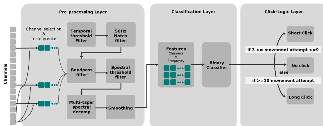
Figure S3. Custom decoder
