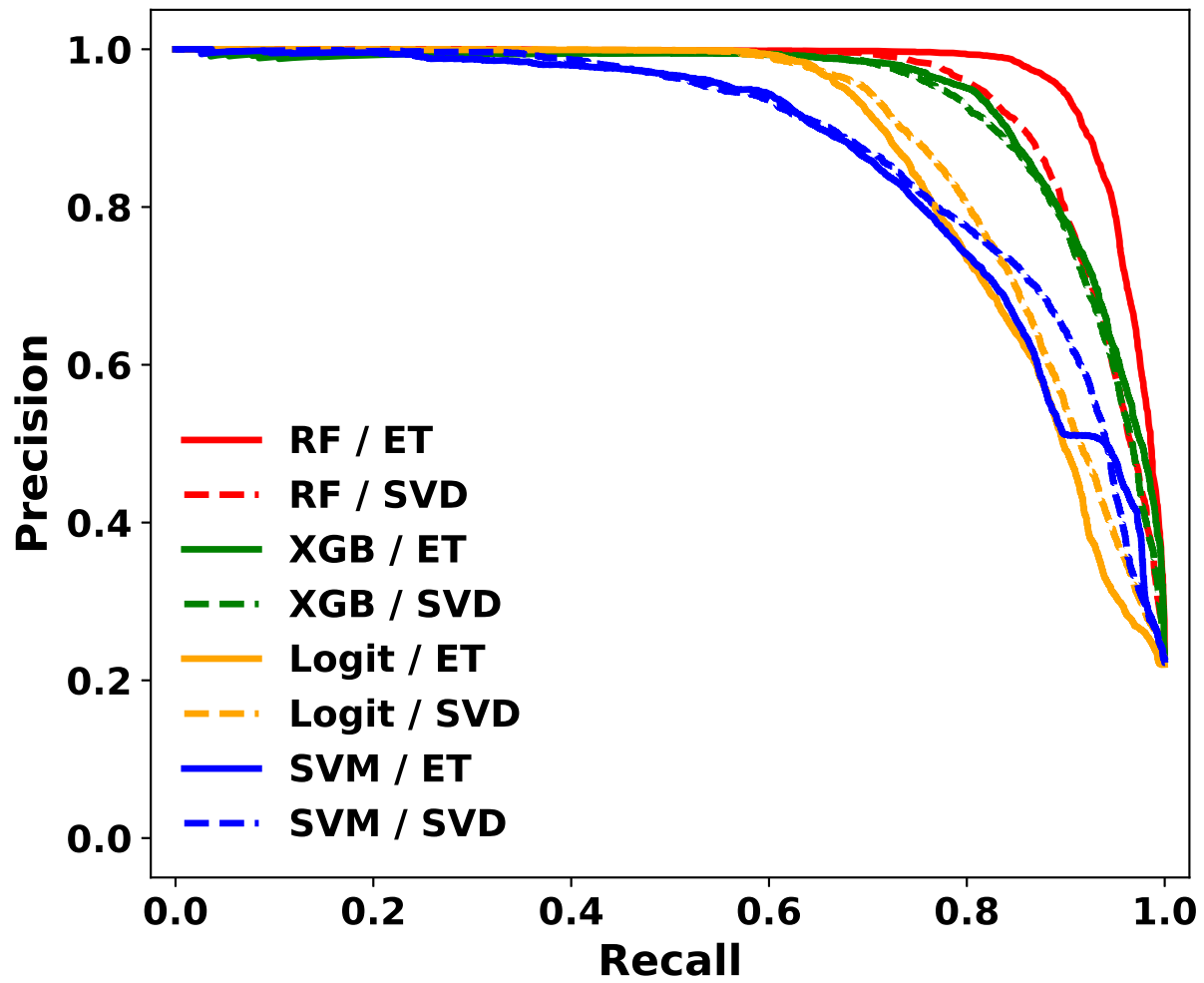
Fig. S2. Classifier P-R performance across many classifier algorithms. Validation set selected from known IO accounts and negatively labeled Snorkel data.
