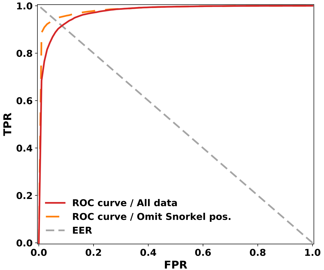
Fig. S5. RF / ET classifier receiver operating characteristic (ROC) performance: true positive rate (TPR, a.k.a. recall) versus false positive rate (FPR); all data (—), and Snorkel positives omitted (---). Classifier EER is determined by the point at which 1 - \text{TPR} = \text{FPR} (dashed gray curve, ---).
