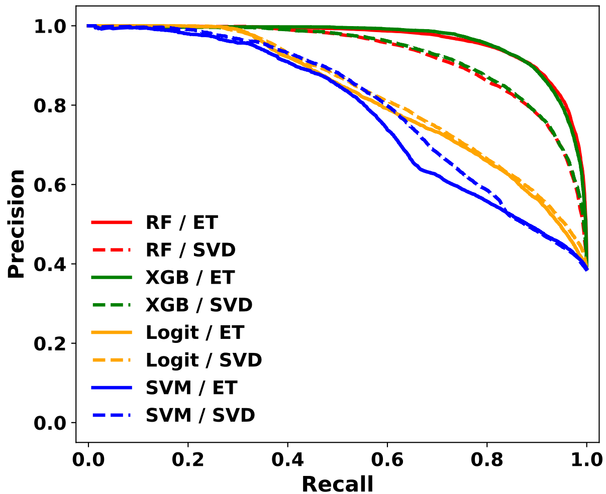
Fig. S3. Classifier P-R performance across many classifier algorithms. Validation set selected from all data.
