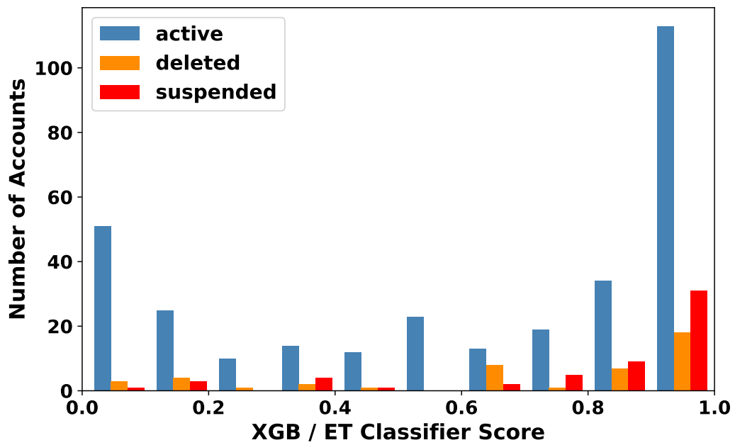
Fig. S8. Classifier score histograms (xgBoost/Extra-Trees) for active, suspended, and deleted accounts in the French narrative network.
