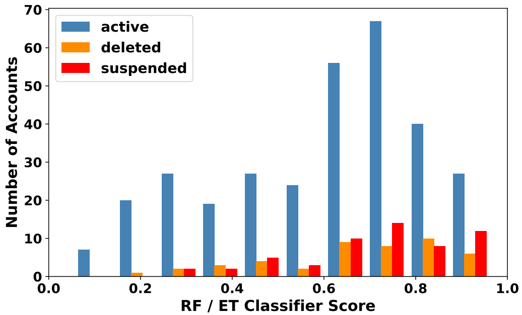
Fig. S7. Classifier score histograms (Random Forest/Extra-Trees) for active, suspended, and deleted accounts in the French narrative network.
