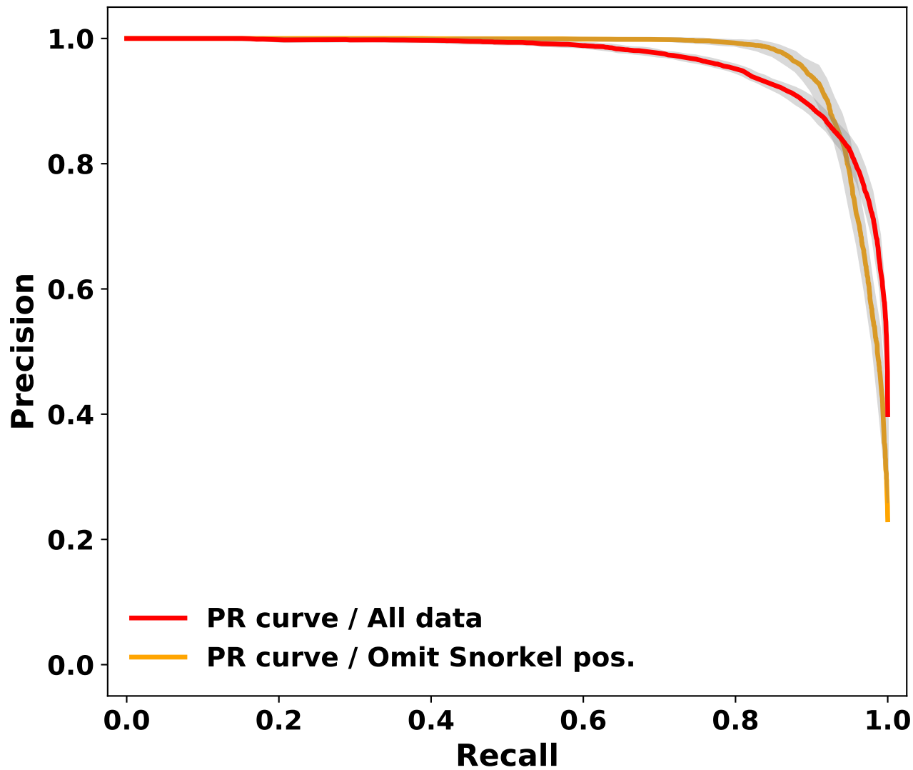
Fig. S4. RF / ET classifier precision–recall (P-R) performance with cross-validation error over twenty 90 : 10 splits; all data (—), and Snorkel positives omitted (—). Maximum standard deviation (gray region, —) is 0.016 and 0.032, respectively.
