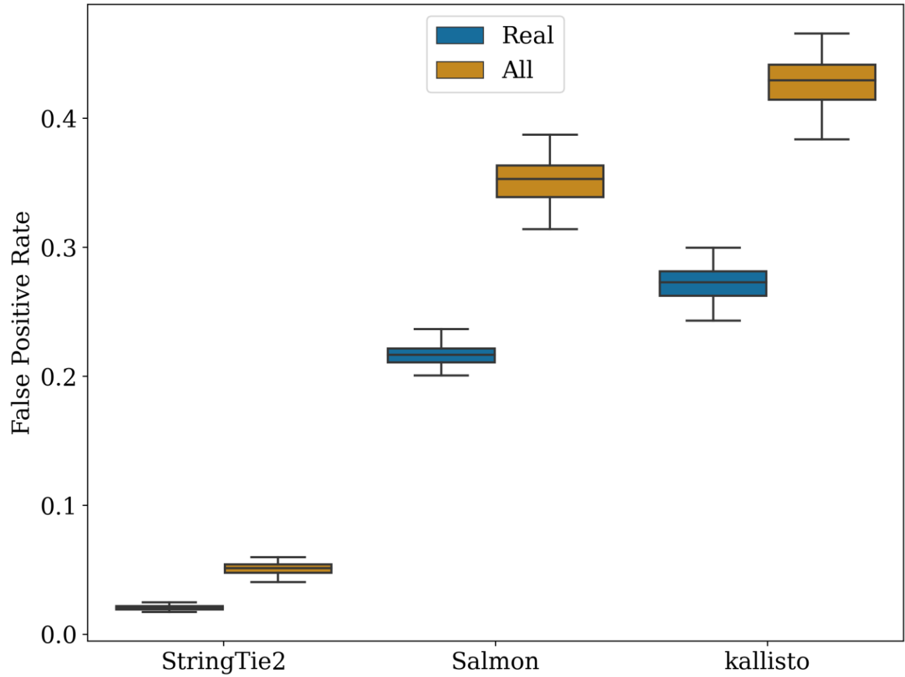
Supplementary Figure 10. False Positive Rate (FPR) for gene quantifications across 30 simulated samples representing 3 simulated tissues. Each method was evaluated separately for each combination of real and noisy reads.
