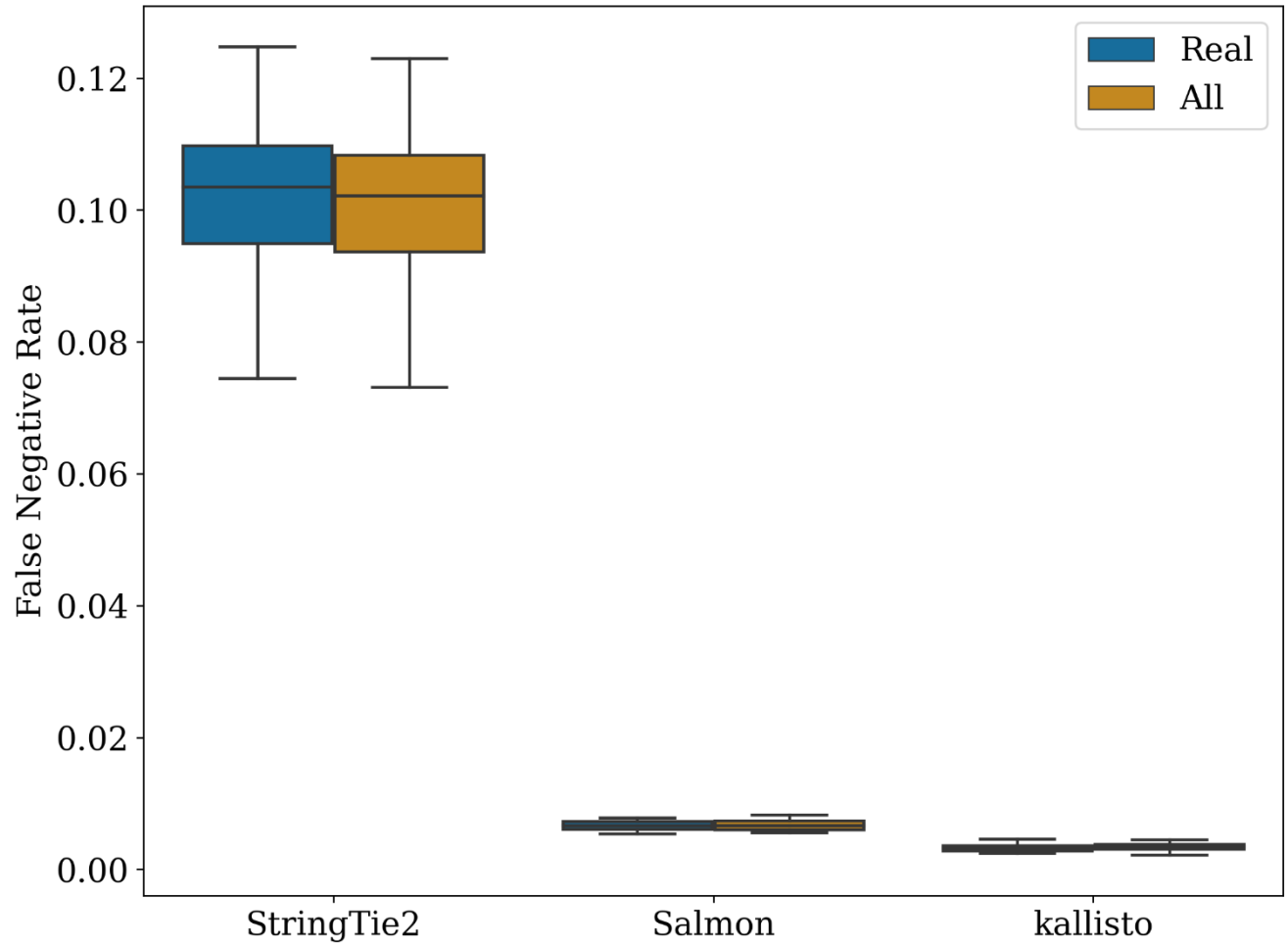
Supplementary Figure 11. False Negative Rate (FNR) for gene quantifications across 30 simulated samples representing 3 simulated tissues. Each method was evaluated separately for each combination of real and noisy reads.
