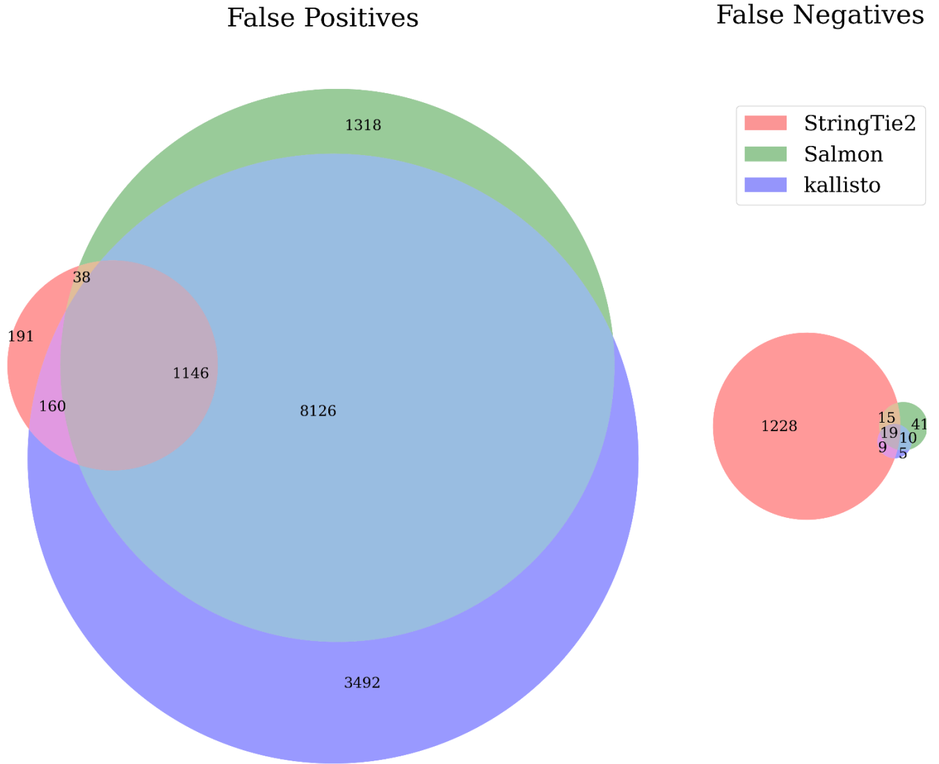
Supplementary Figure 12. False gene predictions. Overlaps between StringTie2, Salmon and Kallisto in reported FP and FN genes in the presence of splicing, intronic and intergenic noise. Average values are reported across 30 simulated experiments.
