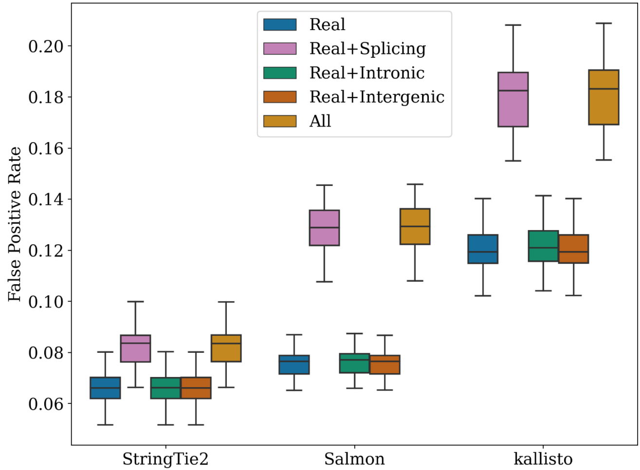
Supplementary Figure 7. False Positive Rate (FPR) for transcript quantifications across 30 simulated samples representing 3 simulated tissues. Each method was evaluated separately for each combination of real and noisy reads.
