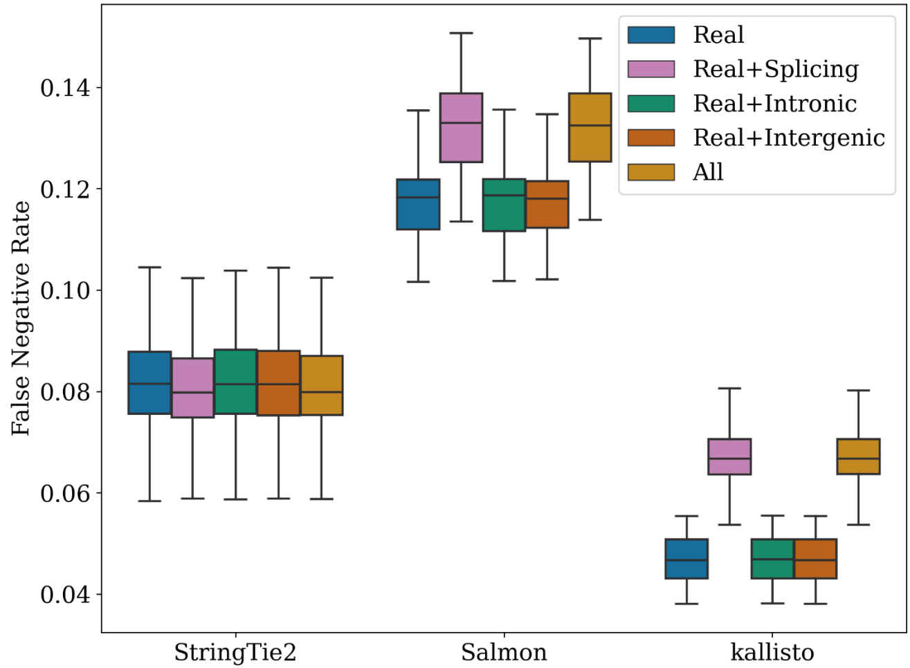
Supplementary Figure 8. False Negative Rate (FNR) for transcript quantifications across 30 simulated samples representing 3 simulated tissues. Each method was evaluated separately for each combination of real and noisy reads.
