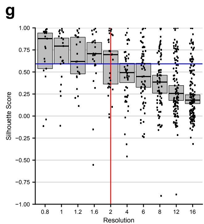
With 50 percent of cells subsampled per iteration
