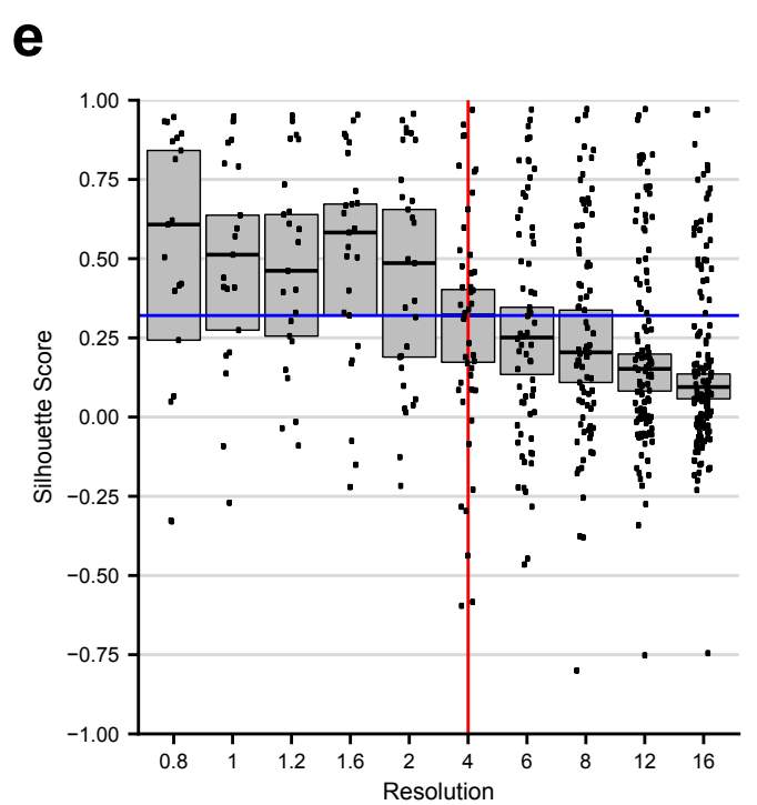
With 20 percent of cells subsampled per iteration
