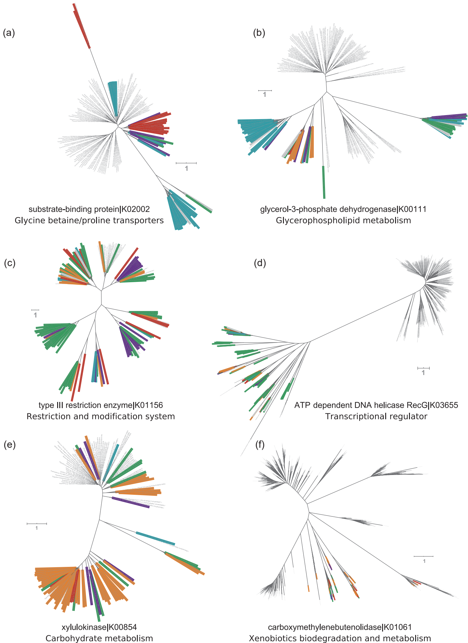
Fig S13. Gene trees of gene families that have undergone HGT with habitat-specific activity. Leaf names shown in color are genes found in the HGT inference. Different colors represent various environmental sources of sequences, the color code using the same scheme as in Figure 5b.
