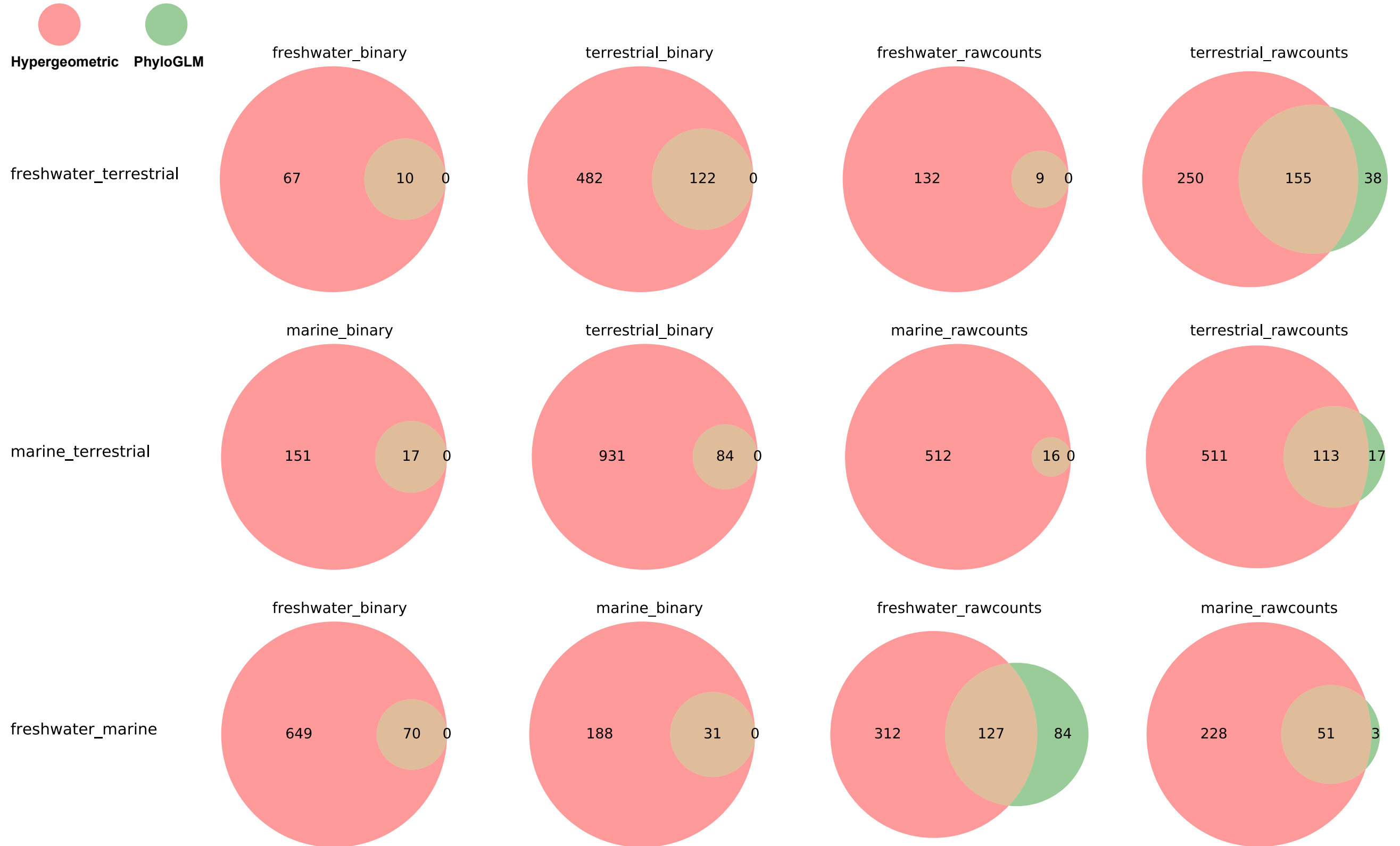
Fig. S5. Number of significant KEGG orthologies predicted by Hypergeometric test and PhyloGLM including presence/absence version (binary) and copy numbers version (rawcounts). Circles filled by red color represent clusters only found in Hypergeometric test, circles in green color denote cluster only found in PhyloGLM test, and circles filled in yellow indicate overlap cluster in Hypergeometric test and PhyloGLM test. The numbers in circles refer to cluster counts.
