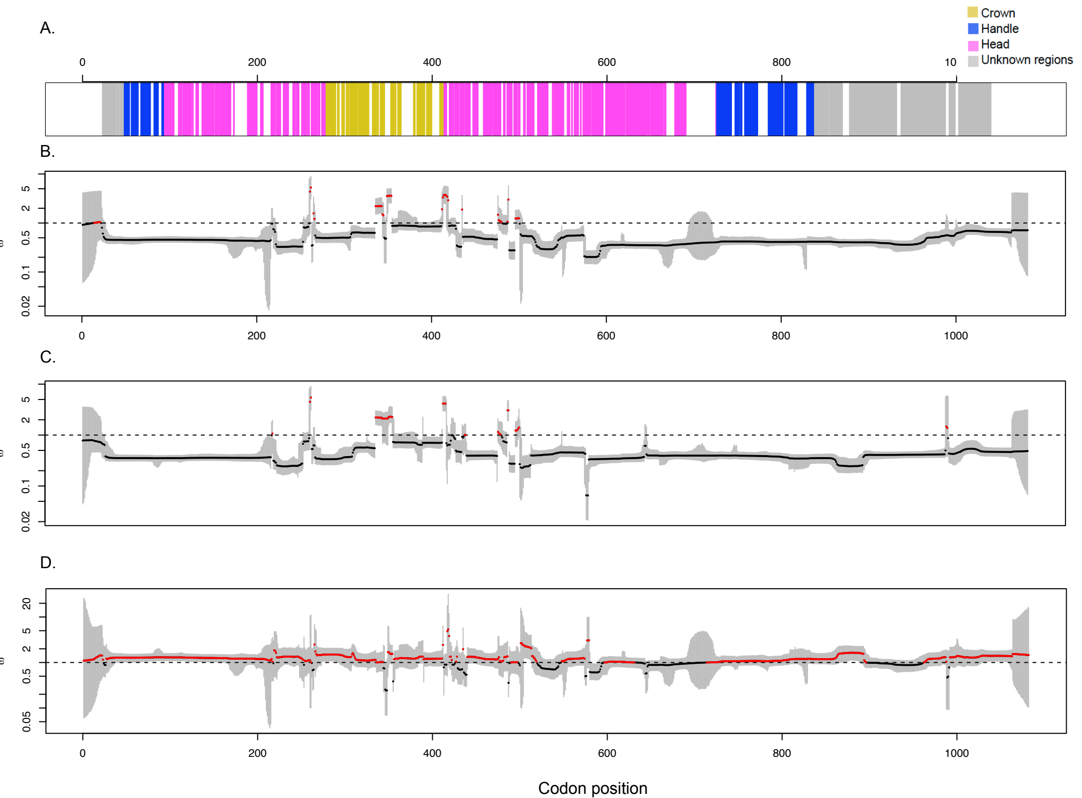
Suppl. Fig. 7. Analyses of positions under selective pressure in the babA gene of strains from the Americas and other continents using GenomegaMap. a) Known domains of BabA [55]; b) omega values for each position of babA in strains from the Americas; c) omega values for each position of babA in strains from the other continents; d) America/non-America ratio of omega values showing positive pressure is higher in most regions of the gene in American strains relative to non-American strains.
