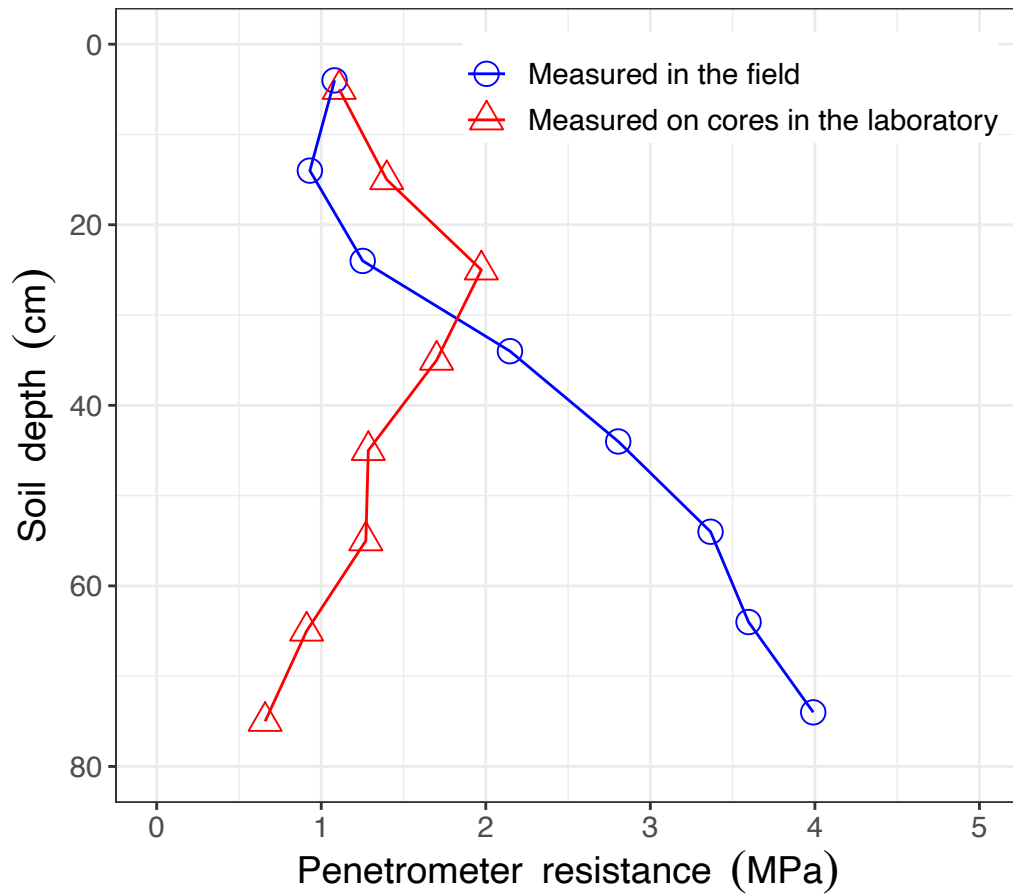
Figure S1. A comparison of penrometer resistance measured in the field with penrometer resistance measured in the laboratory on cores taken in the field
