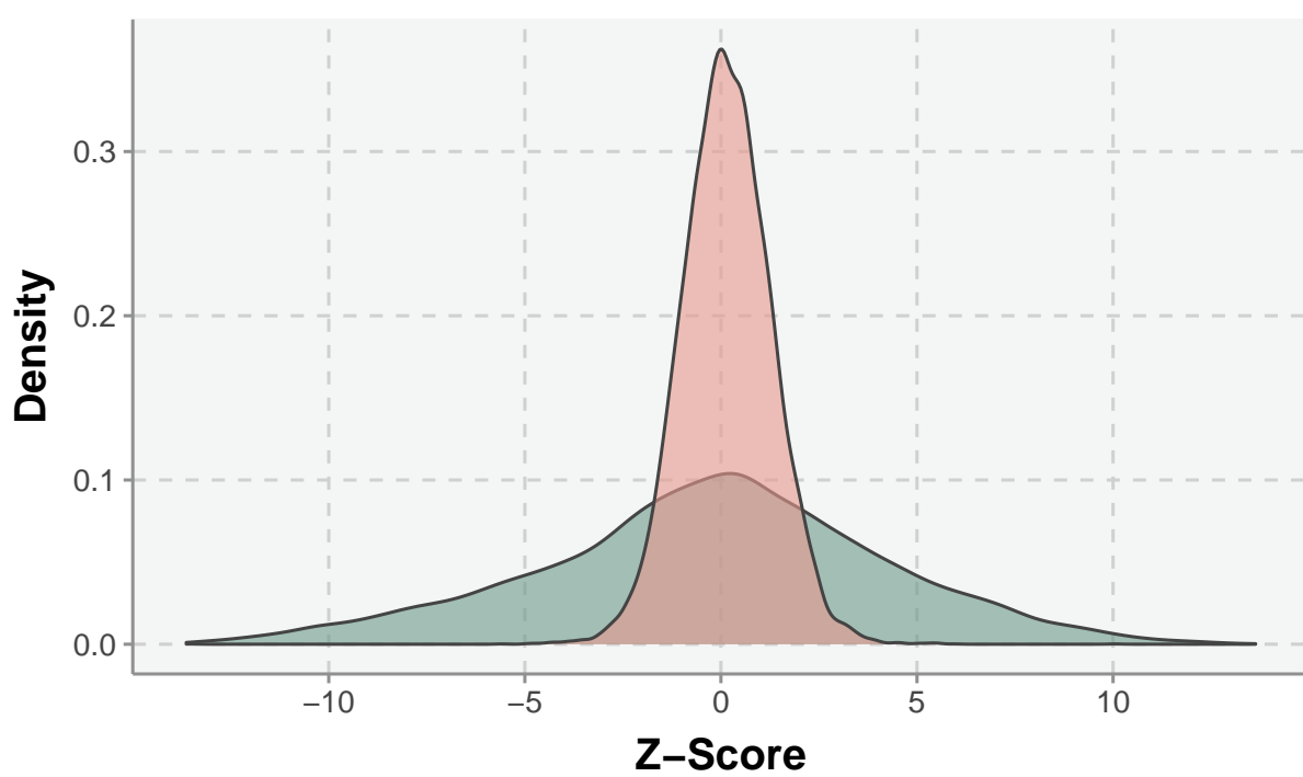
LBD Meta-Analysis
