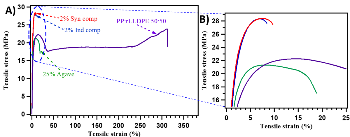
Figure S1: A) Stress-strain curve of PP:rLLDPE (50:50), 25% agave and the composite prepared with 2% synthesized compatibilizer (Syn Comp) and 2% industrial compatibilizer (Ind Comp) and B) zoom on stress-strain curve.
