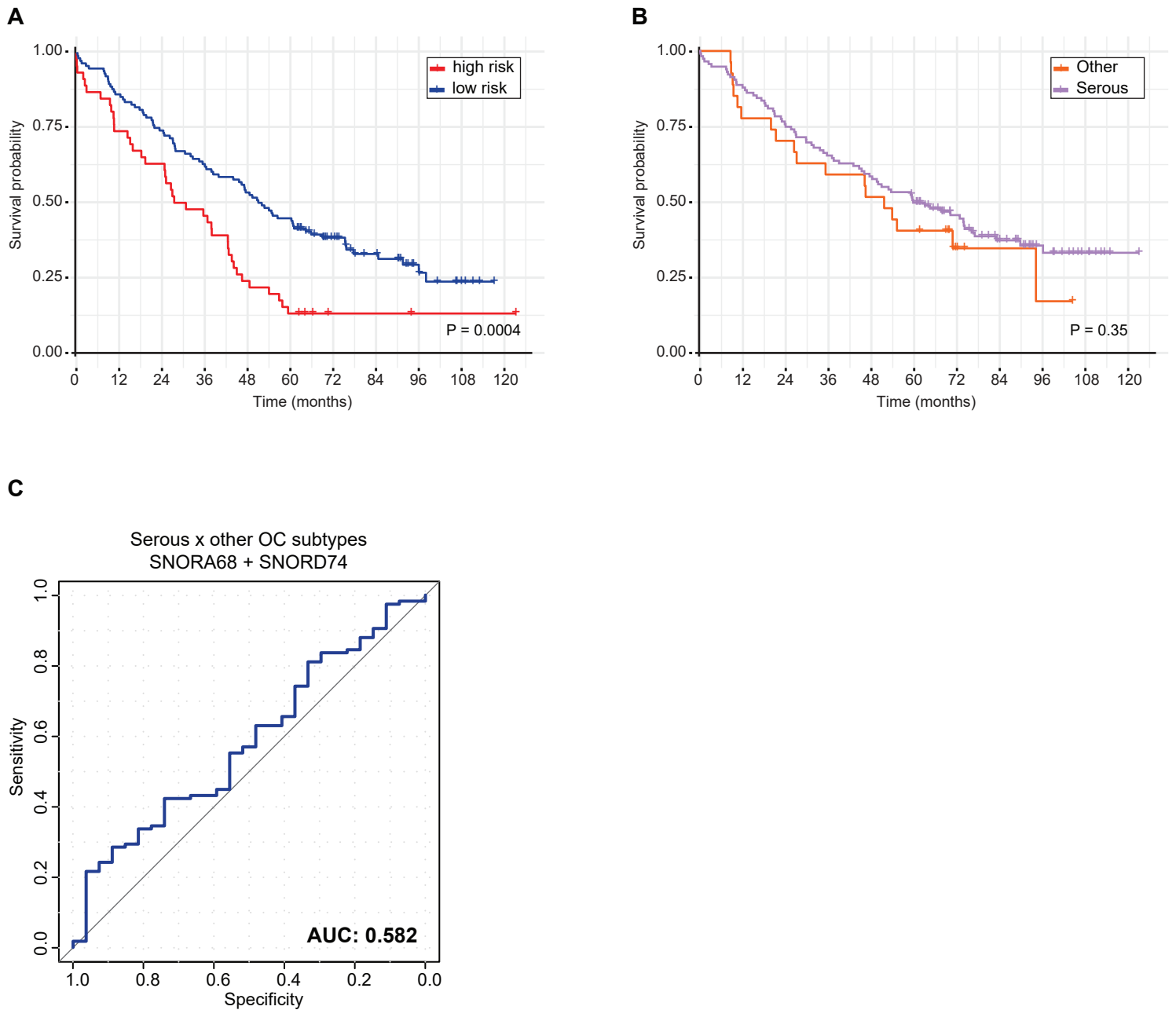
S4 Figure. (A) Survival curve between “high risk” (red) and “low risk” (blue) in serous adenocarcinoma subtype. (B) Survival curve between serous adenocarcinoma and other OC subtypes. (C) AUC/ROC curve of combination of SNORA68 and SNORD74 in serous adenocarcinoma x other OC subtypes. P-values and AUC are presented above.
