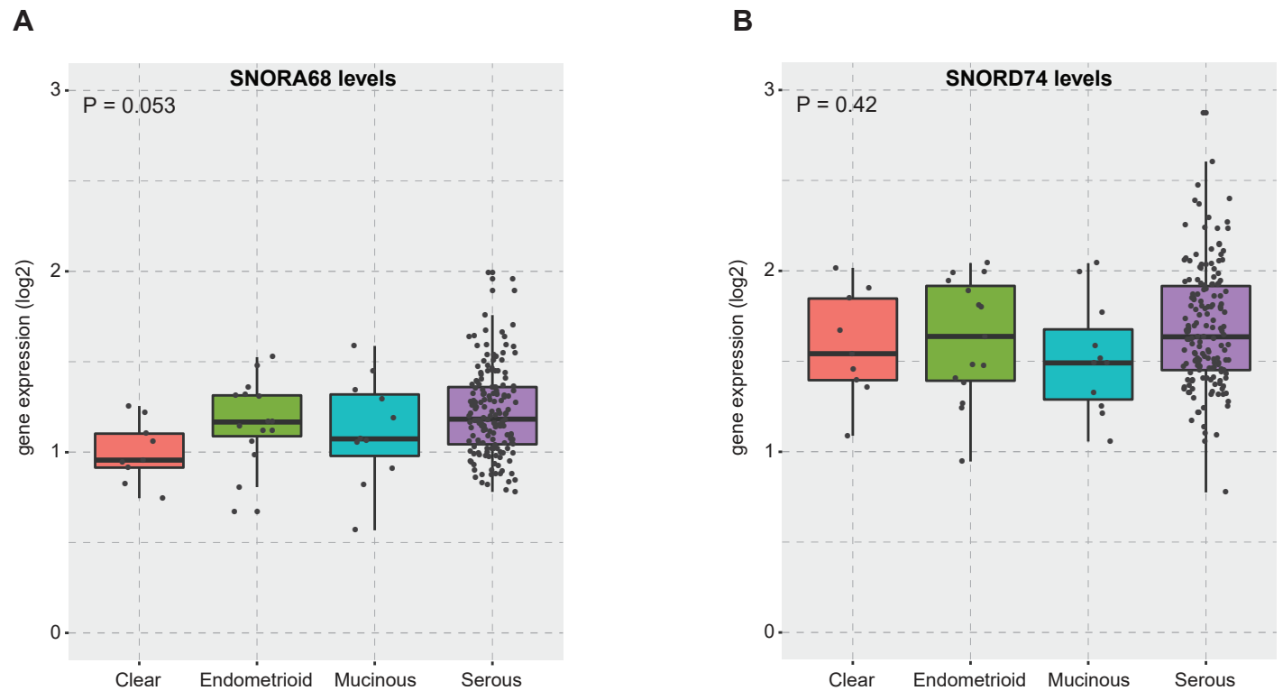
S5 Figure. Gene expression in all OC subtypes for SNORA68 (A), and SNORD74 (B). Values are normalized and provided as log 2 and P-values are presented above.
