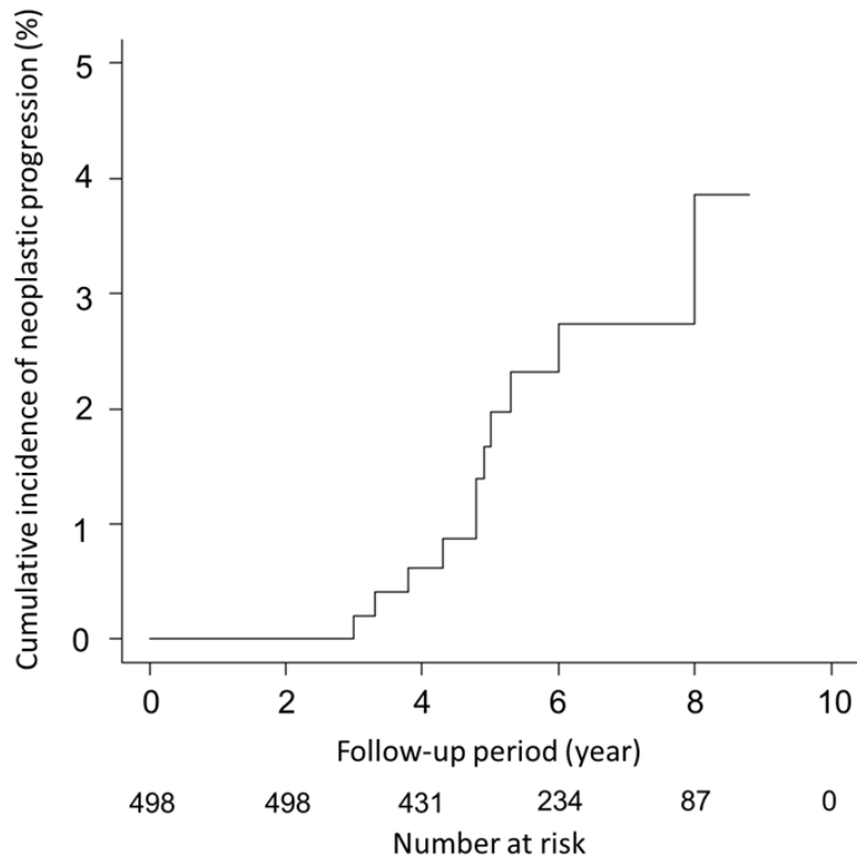
Figure 1. Cumulative incidence of neoplastic progression among 498 patients in the study population. The incidence at 5 years from initial surveillance was 2.0%, and the incidence at 8 years was 3.9%.
