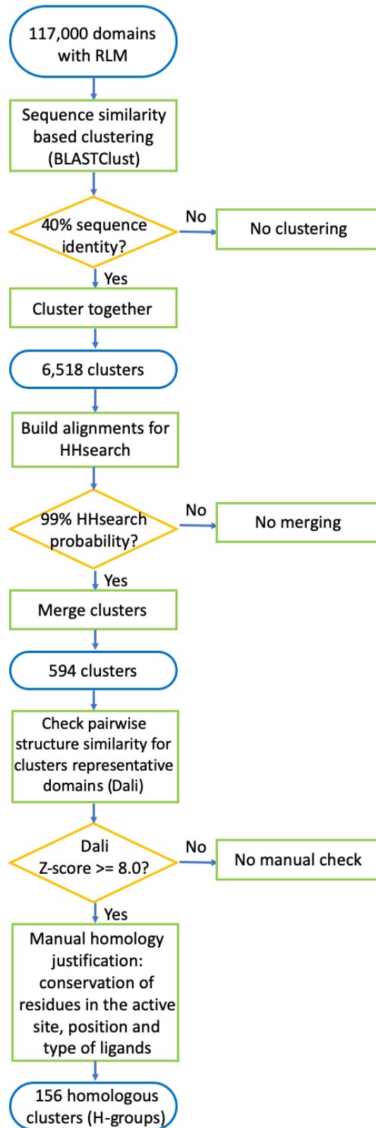
Fig S2. The flowchart of clustering RLM-containing domains into homologous clusters.
