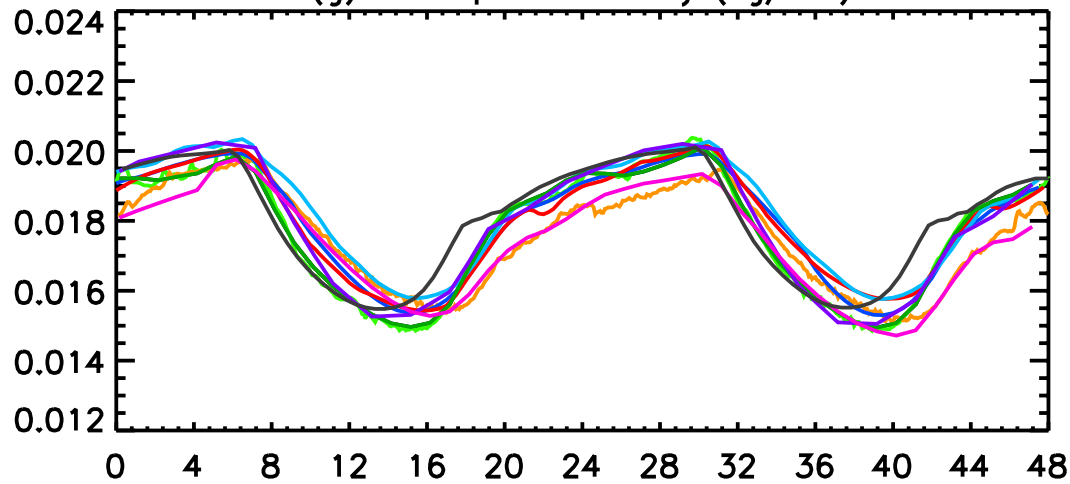
(g) Atmospheric density (kg/m3)
