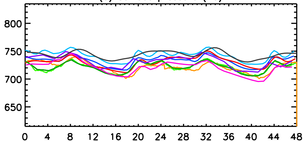
(a) Surface pressure (Pa)
