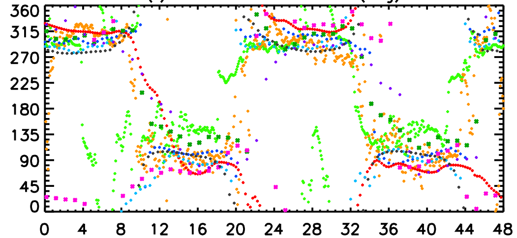
(f) Direction wind is from (deg)
