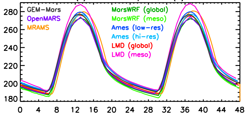
(c) Surface temperature (K)
