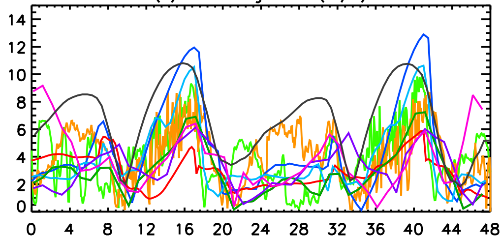
(e) Wind magnitude (m/s)
