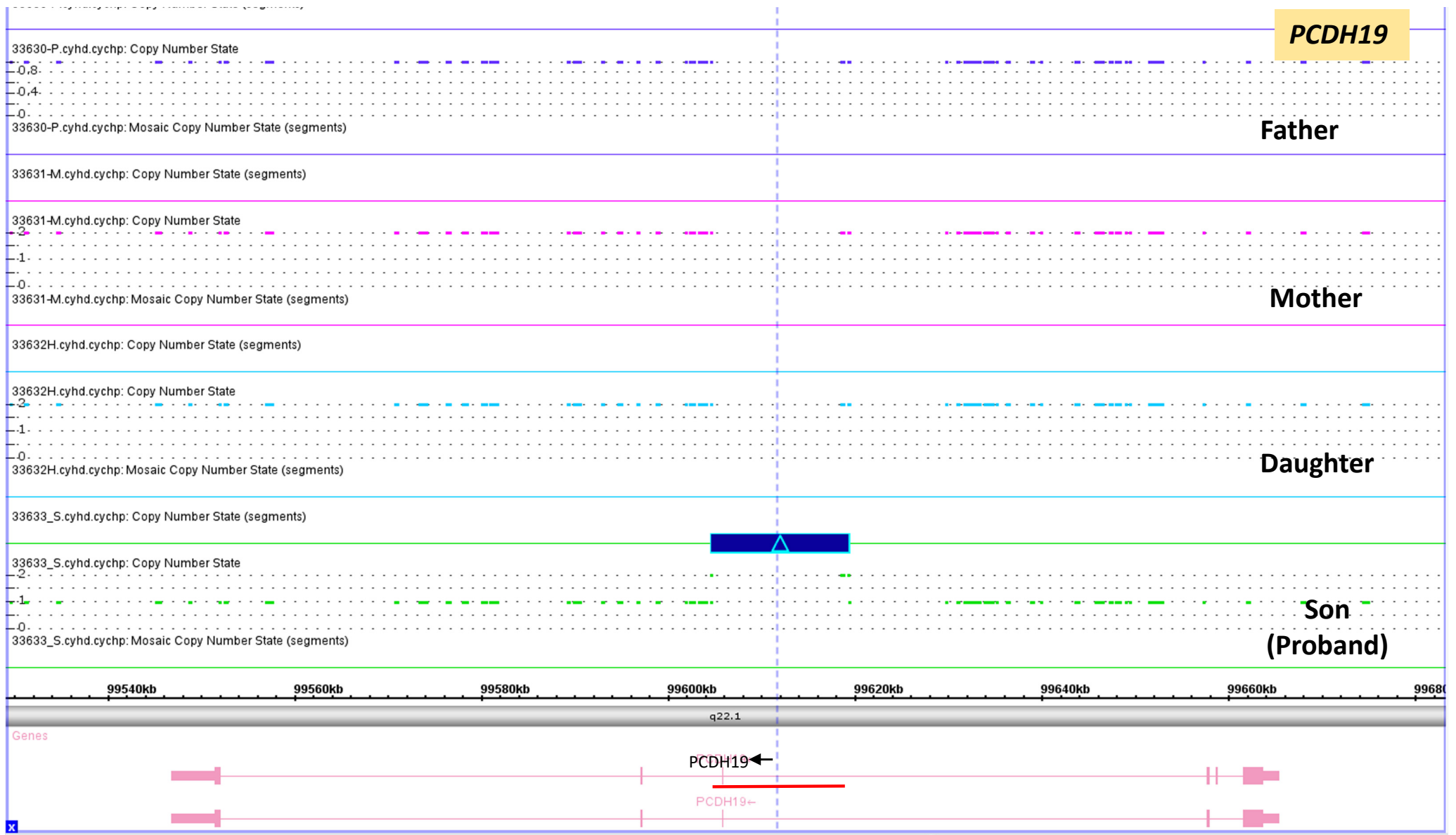
Supplementary Figure S5. Duplication encompassing exon 3 in the PCDH19 gene. The genomic region comprising the PCDH19 gene in the four family members is shown. The region deleted in the proband is marked by a box and a red line. The arrow indicates the direction of transcription.
